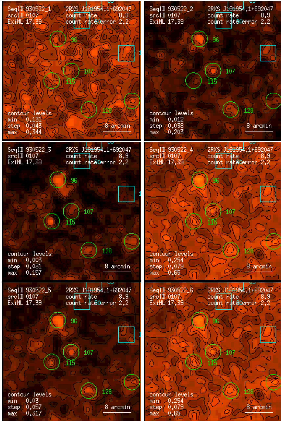
Figure 107: RASS 930522: detection 0107: band rate images, Gaussian filter: (1) PSPC channels 11 – 41, (2) 52 – 90, (3) 91 – 201, (4) 11 – 235, (5) 52 – 201, (6) 11 – 201. Broad band rates in counts/ks. Band rate contour levels in counts/ks/arcmin 2 .
