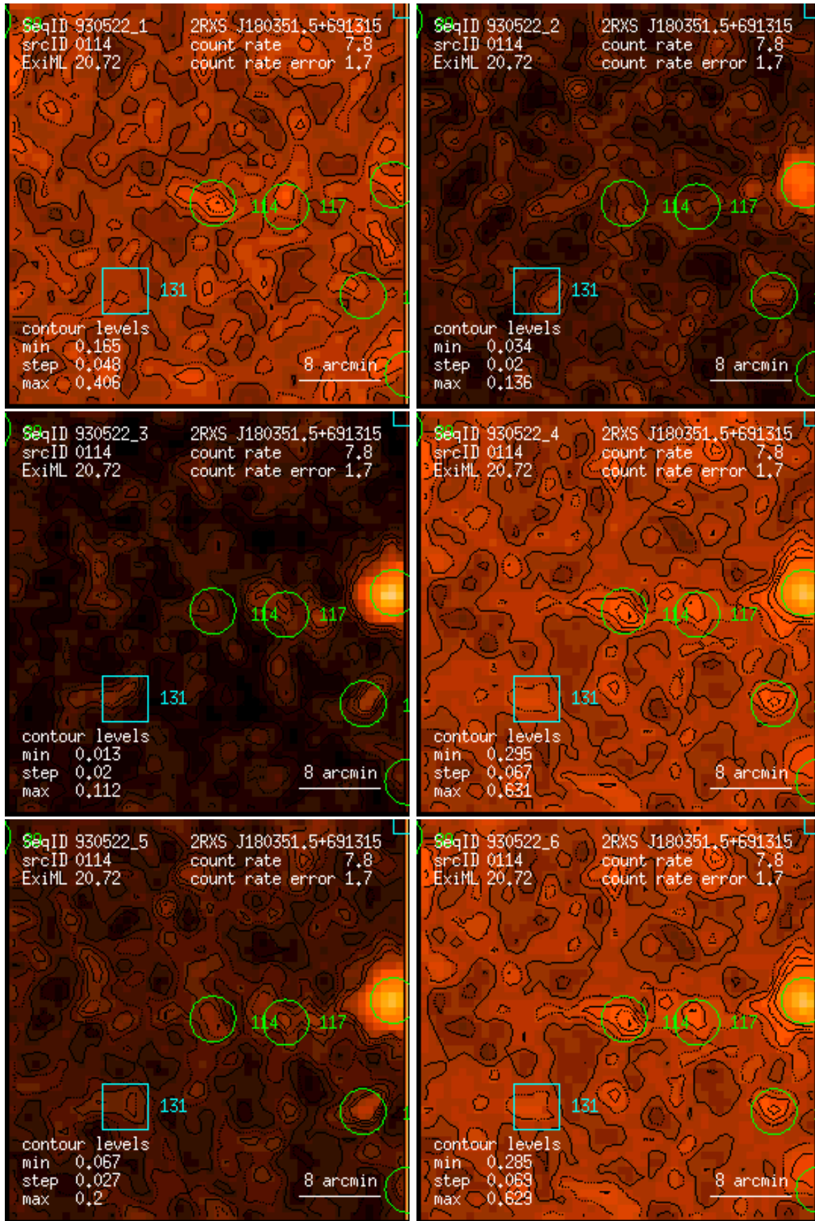
Figure 114: RASS 930522: detection 0114: band rate images, Gaussian filter: (1) PSPC channels 11 – 41, (2) 52 – 90, (3) 91 – 201, (4) 11 – 235, (5) 52 – 201, (6) 11 – 201. Broad band rates in counts/ks. Band rate contour levels in counts/ks/arcmin 2 .
