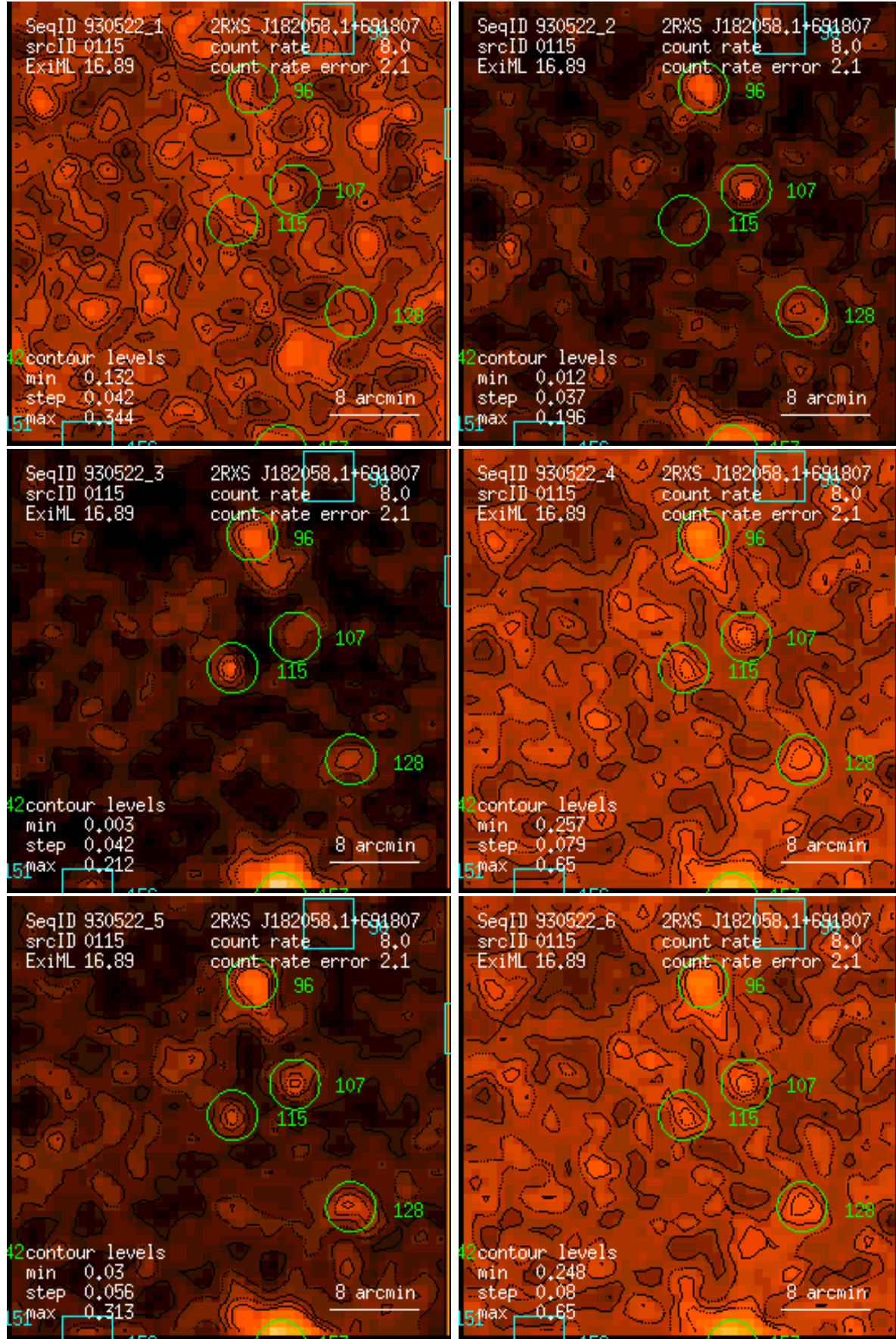
Figure 115: RASS 930522: detection 0115: band rate images, Gaussian filter: (1) PSPC channels 11 – 41, (2) 52 – 90, (3) 91 – 201, (4) 11 – 235, (5) 52 – 201, (6) 11 – 201. Broad band rates in counts/ks. Band rate contour levels in counts/ks/arcmin 2 .
