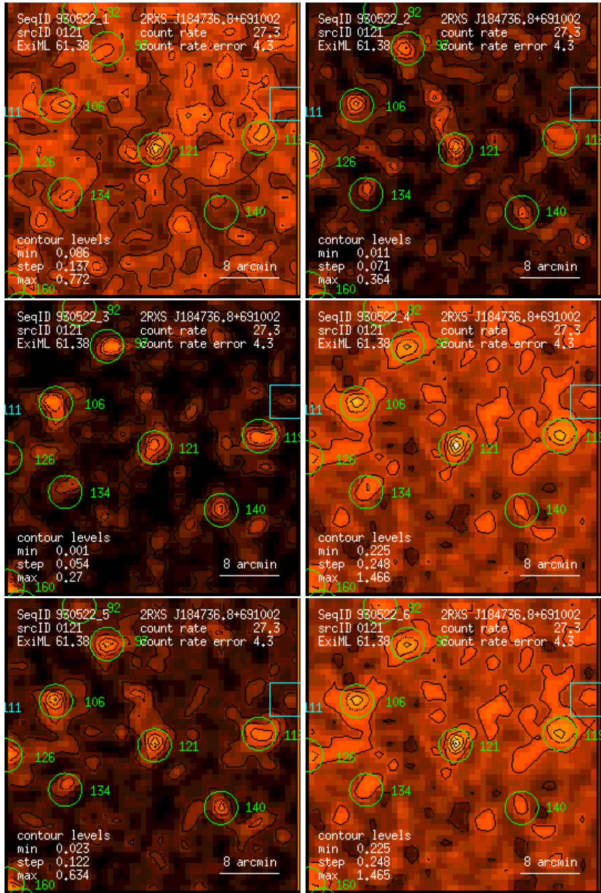
Figure 121: RASS 930522: detection 0121: band rate images, Gaussian filter: (1) PSPC channels 11 – 41, (2) 52 – 90, (3) 91 – 201, (4) 11 – 235, (5) 52 – 201, (6) 11 – 201. Broad band rates in counts/ks. Band rate contour levels in counts/ks/arcmin 2 .
