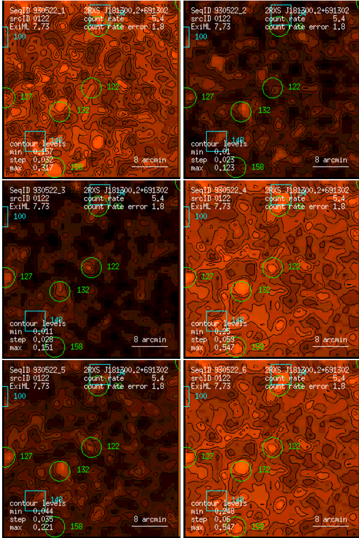
Figure 122: RASS 930522: detection 0122: band rate images, Gaussian filter: (1) PSPC channels 11 – 41, (2) 52 – 90, (3) 91 – 201, (4) 11 – 235, (5) 52 – 201, (6) 11 – 201. Broad band rates in counts/ks. Band rate contour levels in counts/ks/arcmin 2 .
