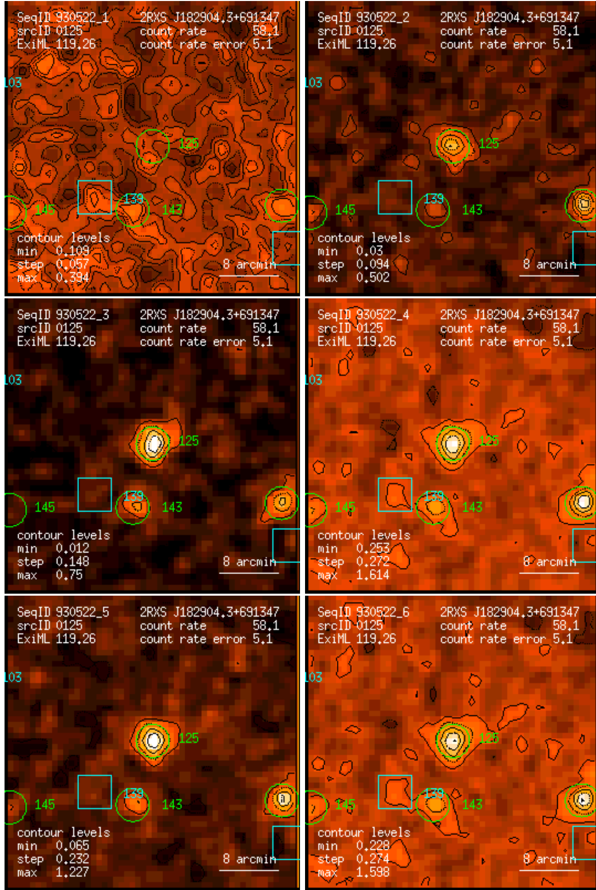
Figure 125: RASS 930522: detection 0125: band rate images, Gaussian filter: (1) PSPC channels 11 – 41, (2) 52 – 90, (3) 91 – 201, (4) 11 – 235, (5) 52 – 201, (6) 11 – 201. Broad band rates in counts/ks. Band rate contour levels in counts/ks/arcmin 2 .
