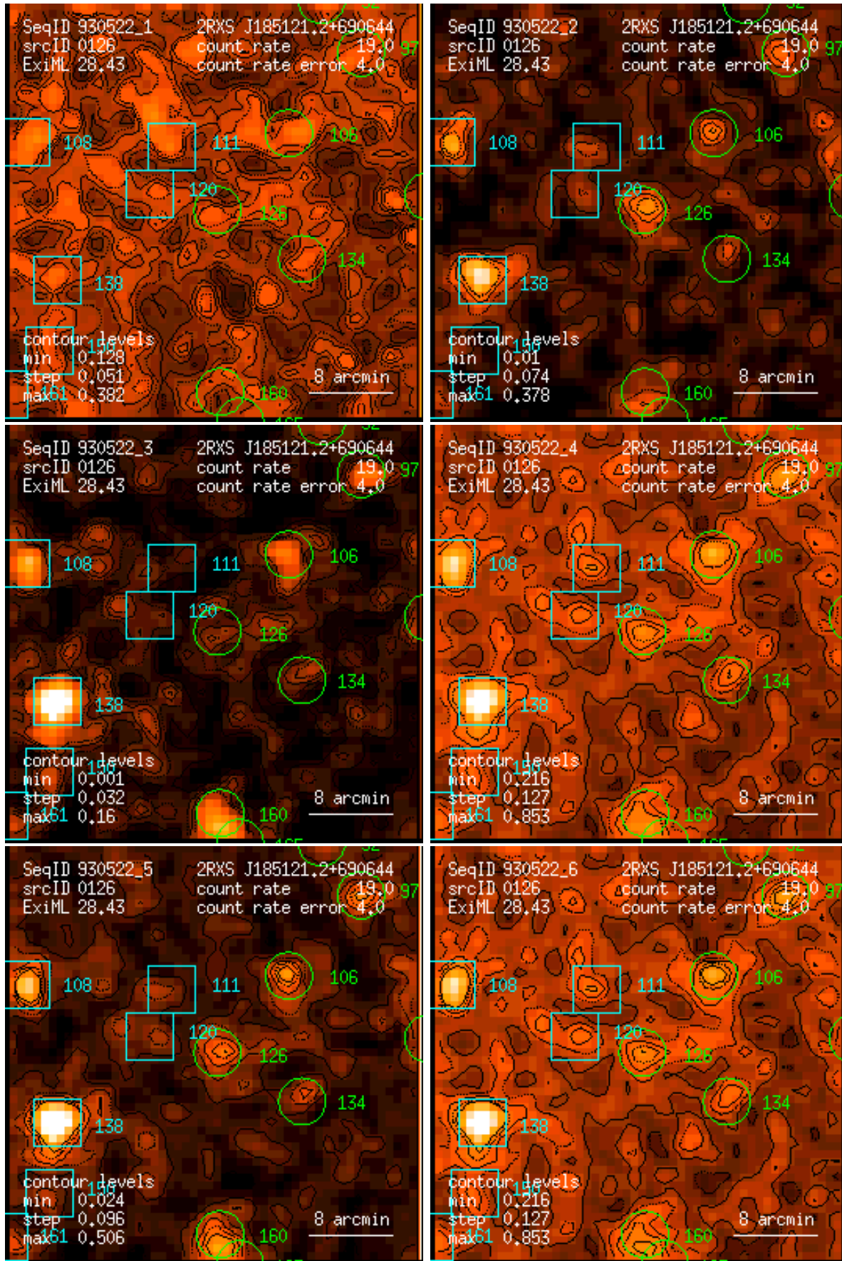
Figure 126: RASS 930522: detection 0126: band rate images, Gaussian filter: (1) PSPC channels 11 – 41, (2) 52 – 90, (3) 91 – 201, (4) 11 – 235, (5) 52 – 201, (6) 11 – 201. Broad band rates in counts/ks. Band rate contour levels in counts/ks/arcmin 2 .
