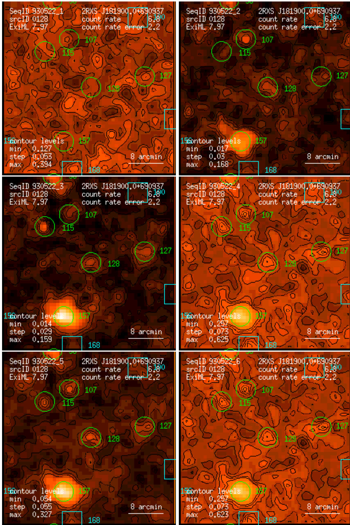
Figure 128: RASS 930522: detection 0128: band rate images, Gaussian filter: (1) PSPC channels 11 – 41, (2) 52 – 90, (3) 91 – 201, (4) 11 – 235, (5) 52 – 201, (6) 11 – 201. Broad band rates in counts/ks. Band rate contour levels in counts/ks/arcmin 2 .
