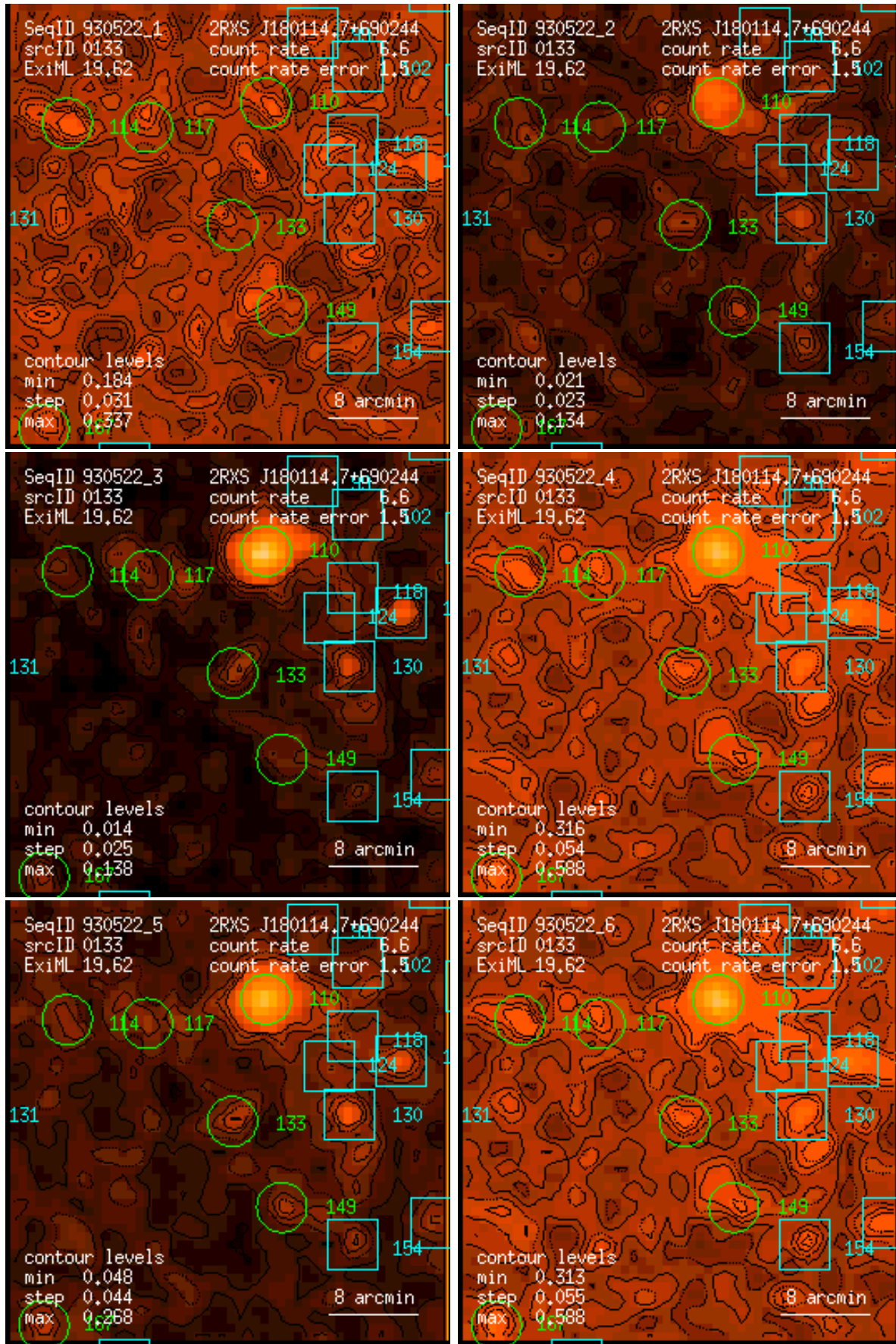
Figure 133: RASS 930522: detection 0133: band rate images, Gaussian filter: (1) PSPC channels 11 – 41, (2) 52 – 90, (3) 91 – 201, (4) 11 – 235, (5) 52 – 201, (6) 11 – 201. Broad band rates in counts/ks. Band rate contour levels in counts/ks/arcmin 2 .
