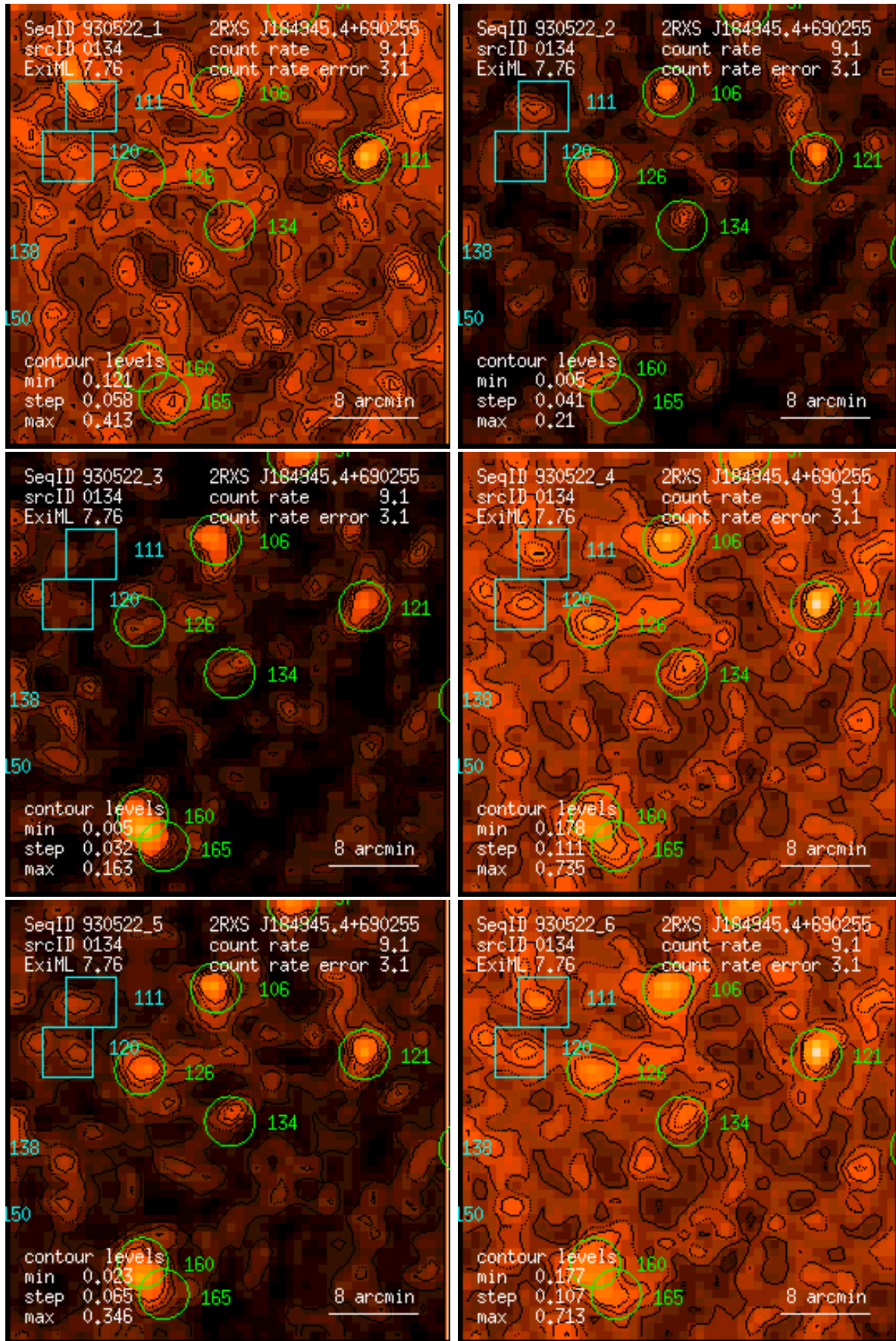
Figure 134: RASS 930522: detection 0134: band rate images, Gaussian filter: (1) PSPC channels 11 – 41, (2) 52 – 90, (3) 91 – 201, (4) 11 – 235, (5) 52 – 201, (6) 11 – 201. Broad band rates in counts/ks. Band rate contour levels in counts/ks/arcmin 2 .
