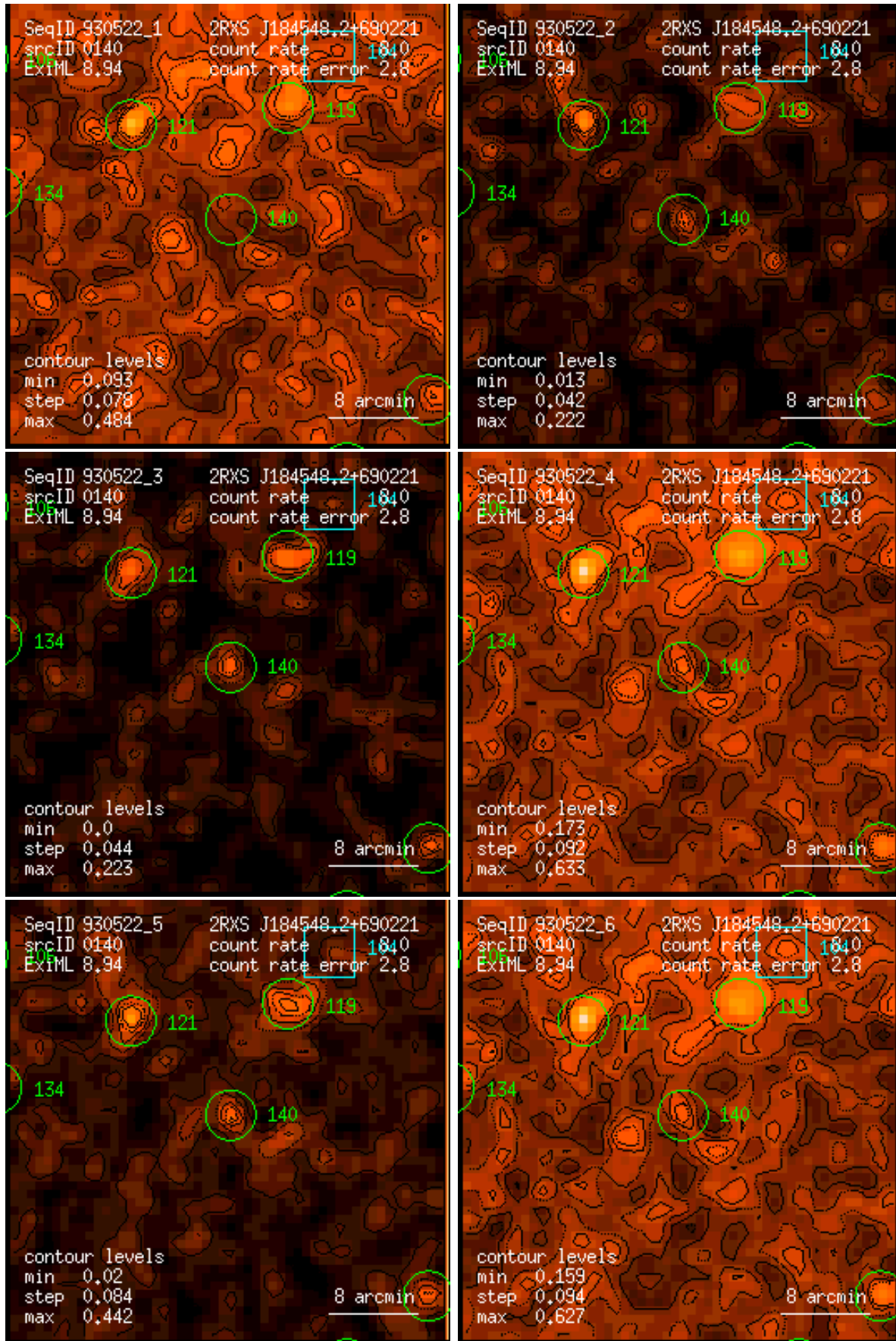
Figure 140: RASS 930522: detection 0140: band rate images, Gaussian filter: (1) PSPC channels 11 – 41, (2) 52 – 90, (3) 91 – 201, (4) 11 – 235, (5) 52 – 201, (6) 11 – 201. Broad band rates in counts/ks. Band rate contour levels in counts/ks/arcmin 2 .
