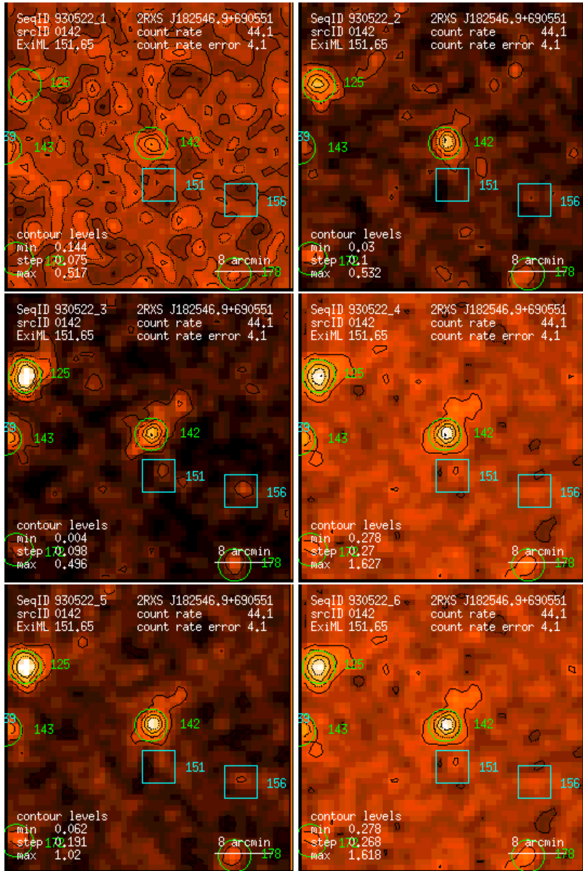
Figure 142: RASS 930522: detection 0142: band rate images, Gaussian filter: (1) PSPC channels 11 – 41, (2) 52 – 90, (3) 91 – 201, (4) 11 – 235, (5) 52 – 201, (6) 11 – 201. Broad band rates in counts/ks. Band rate contour levels in counts/ks/arcmin 2 .
