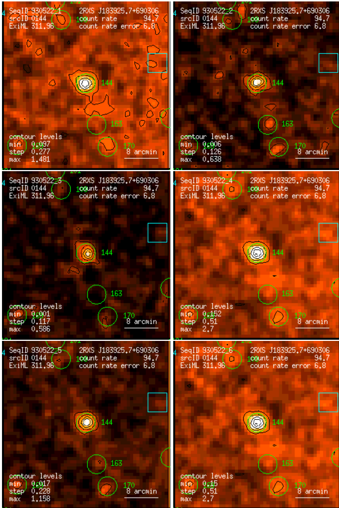
Figure 144: RASS 930522: detection 0144: band rate images, Gaussian filter: (1) PSPC channels 11 – 41, (2) 52 – 90, (3) 91 – 201, (4) 11 – 235, (5) 52 – 201, (6) 11 – 201. Broad band rates in counts/ks. Band rate contour levels in counts/ks/arcmin 2 .
