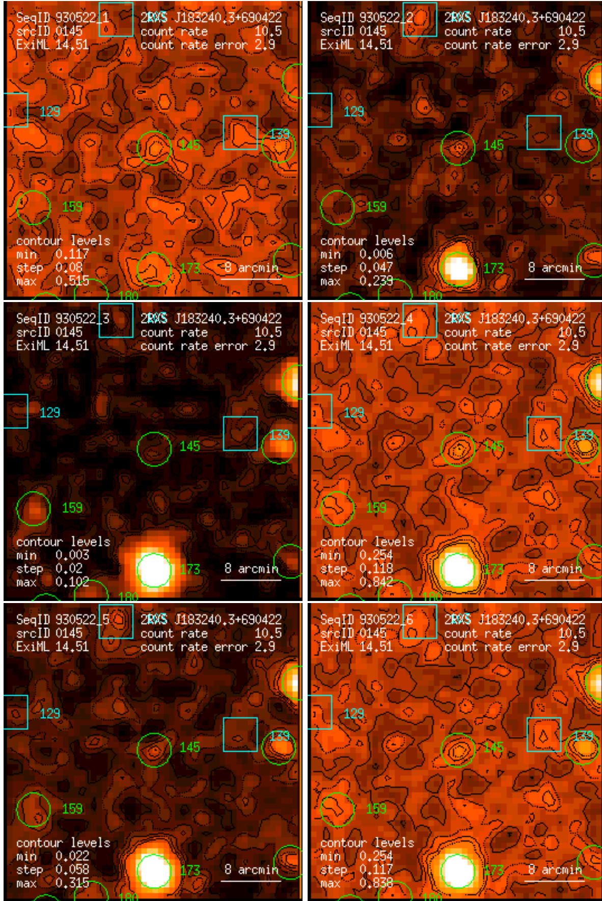
Figure 145: RASS 930522: detection 0145: band rate images, Gaussian filter: (1) PSPC channels 11 – 41, (2) 52 – 90, (3) 91 – 201, (4) 11 – 235, (5) 52 – 201, (6) 11 – 201. Broad band rates in counts/ks. Band rate contour levels in counts/ks/arcmin 2 .
