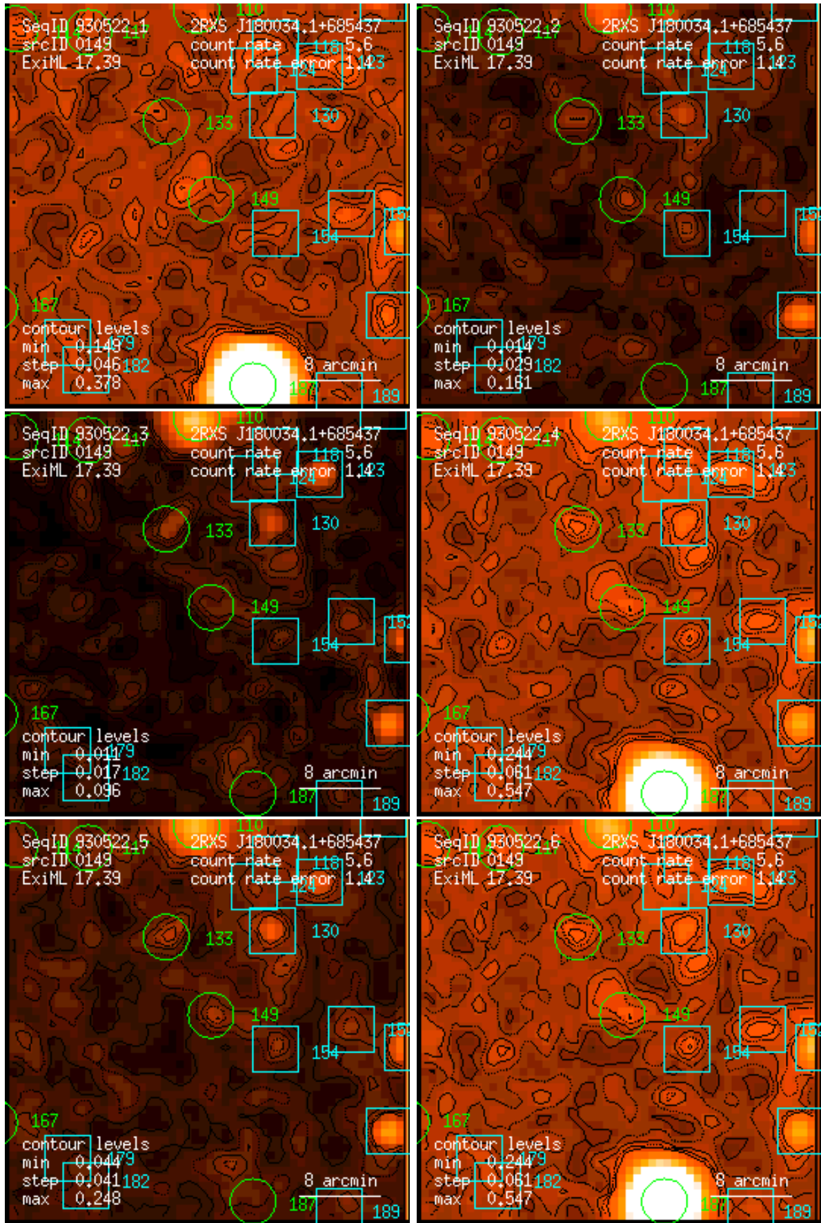
Figure 149: RASS 930522: detection 0149: band rate images, Gaussian filter: (1) PSPC channels 11 – 41, (2) 52 – 90, (3) 91 – 201, (4) 11 – 235, (5) 52 – 201, (6) 11 – 201. Broad band rates in counts/ks. Band rate contour levels in counts/ks/arcmin 2 .
