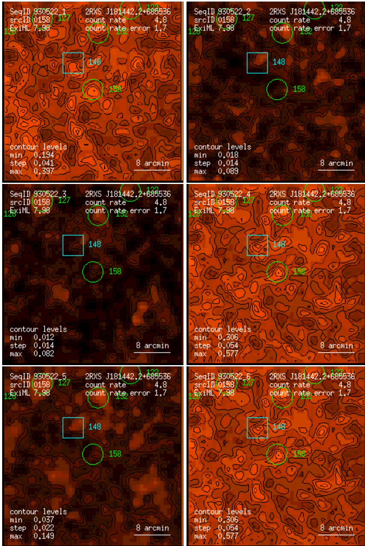
Figure 158: RASS 930522: detection 0158: band rate images, Gaussian filter: (1) PSPC channels 11 – 41, (2) 52 – 90, (3) 91 – 201, (4) 11 – 235, (5) 52 – 201, (6) 11 – 201. Broad band rates in counts/ks. Band rate contour levels in counts/ks/arcmin 2 .
