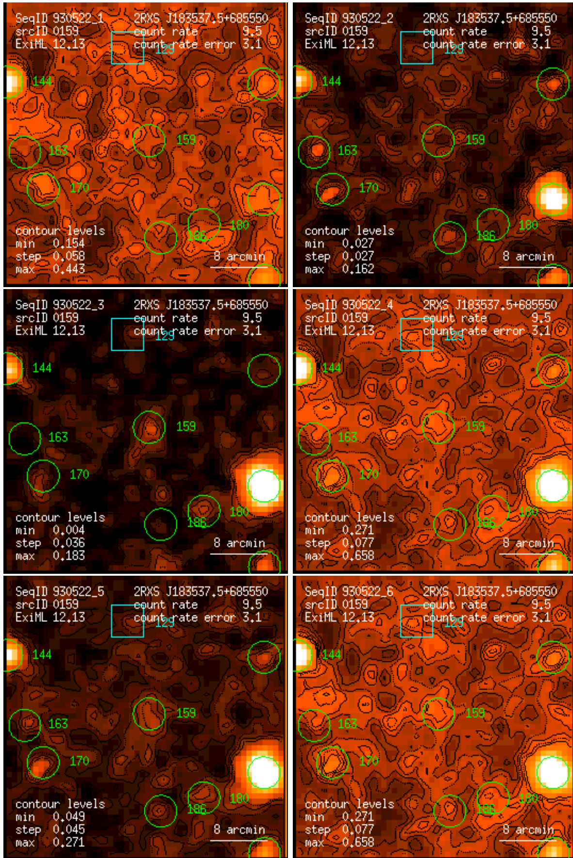
Figure 159: RASS 930522: detection 0159: band rate images, Gaussian filter: (1) PSPC channels 11 – 41, (2) 52 – 90, (3) 91 – 201, (4) 11 – 235, (5) 52 – 201, (6) 11 – 201. Broad band rates in counts/ks. Band rate contour levels in counts/ks/arcmin 2 .
