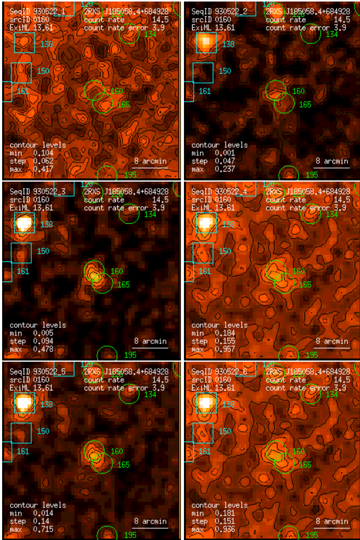
Figure 160: RASS 930522: detection 0160: band rate images, Gaussian filter: (1) PSPC channels 11 – 41, (2) 52 – 90, (3) 91 – 201, (4) 11 – 235, (5) 52 – 201, (6) 11 – 201. Broad band rates in counts/ks. Band rate contour levels in counts/ks/arcmin 2 .
