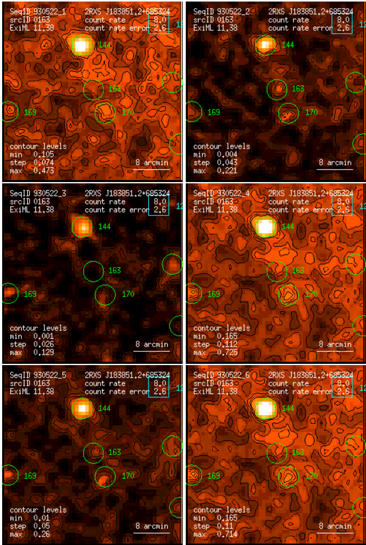
Figure 163: RASS 930522: detection 0163: band rate images, Gaussian filter: (1) PSPC channels 11 – 41, (2) 52 – 90, (3) 91 – 201, (4) 11 – 235, (5) 52 – 201, (6) 11 – 201. Broad band rates in counts/ks. Band rate contour levels in counts/ks/arcmin 2 .
