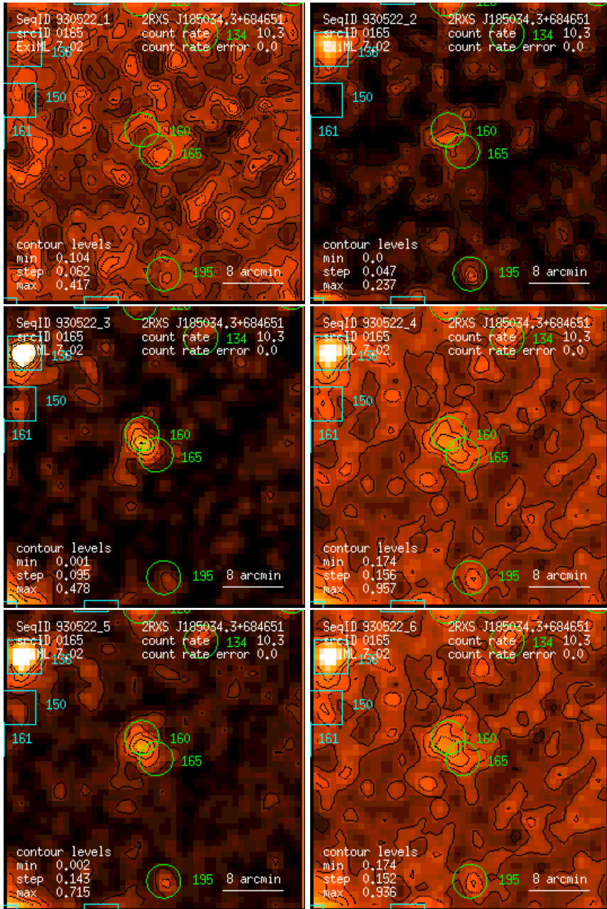
Figure 165: RASS 930522: detection 0165: band rate images, Gaussian filter: (1) PSPC channels 11 – 41, (2) 52 – 90, (3) 91 – 201, (4) 11 – 235, (5) 52 – 201, (6) 11 – 201. Broad band rates in counts/ks. Band rate contour levels in counts/ks/arcmin 2 .
