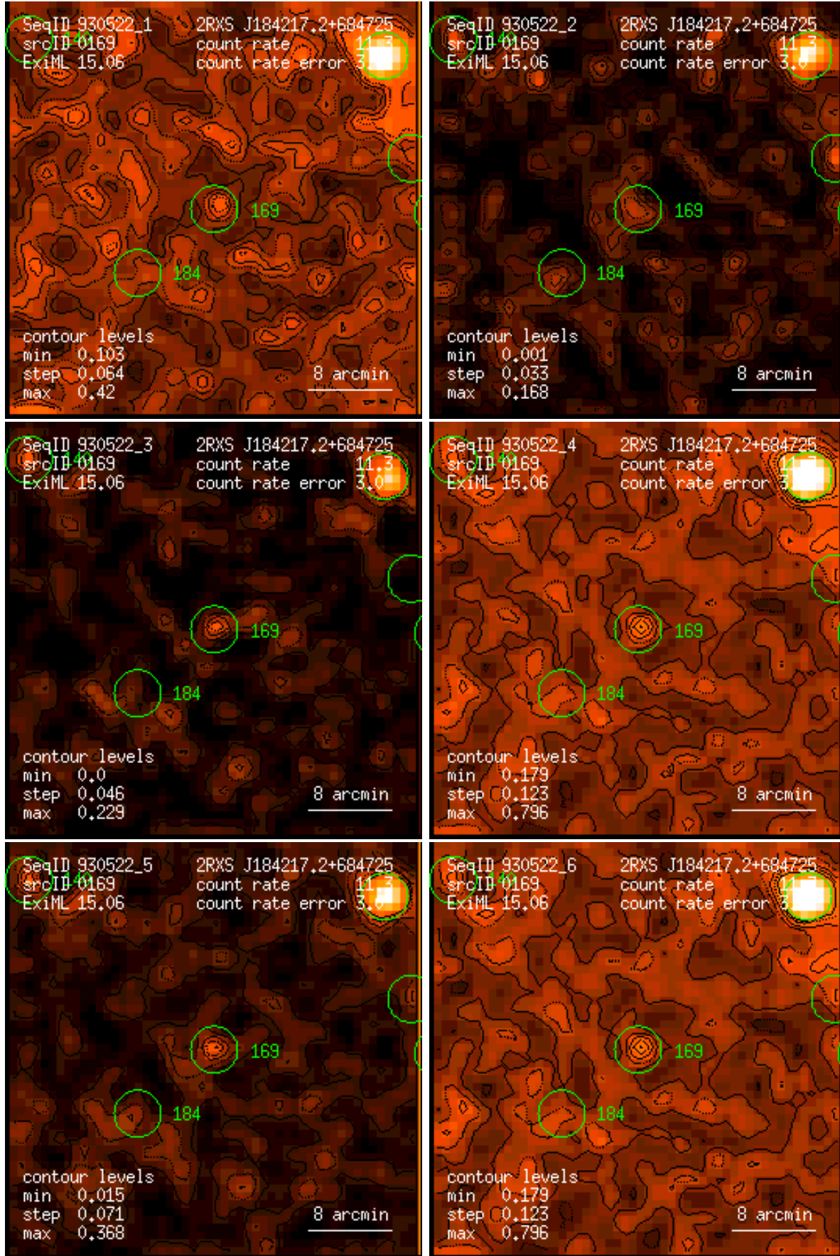
Figure 169: RASS 930522: detection 0169: band rate images, Gaussian filter: (1) PSPC channels 11 – 41, (2) 52 – 90, (3) 91 – 201, (4) 11 – 235, (5) 52 – 201, (6) 11 – 201. Broad band rates in counts/ks. Band rate contour levels in counts/ks/arcmin 2 .
