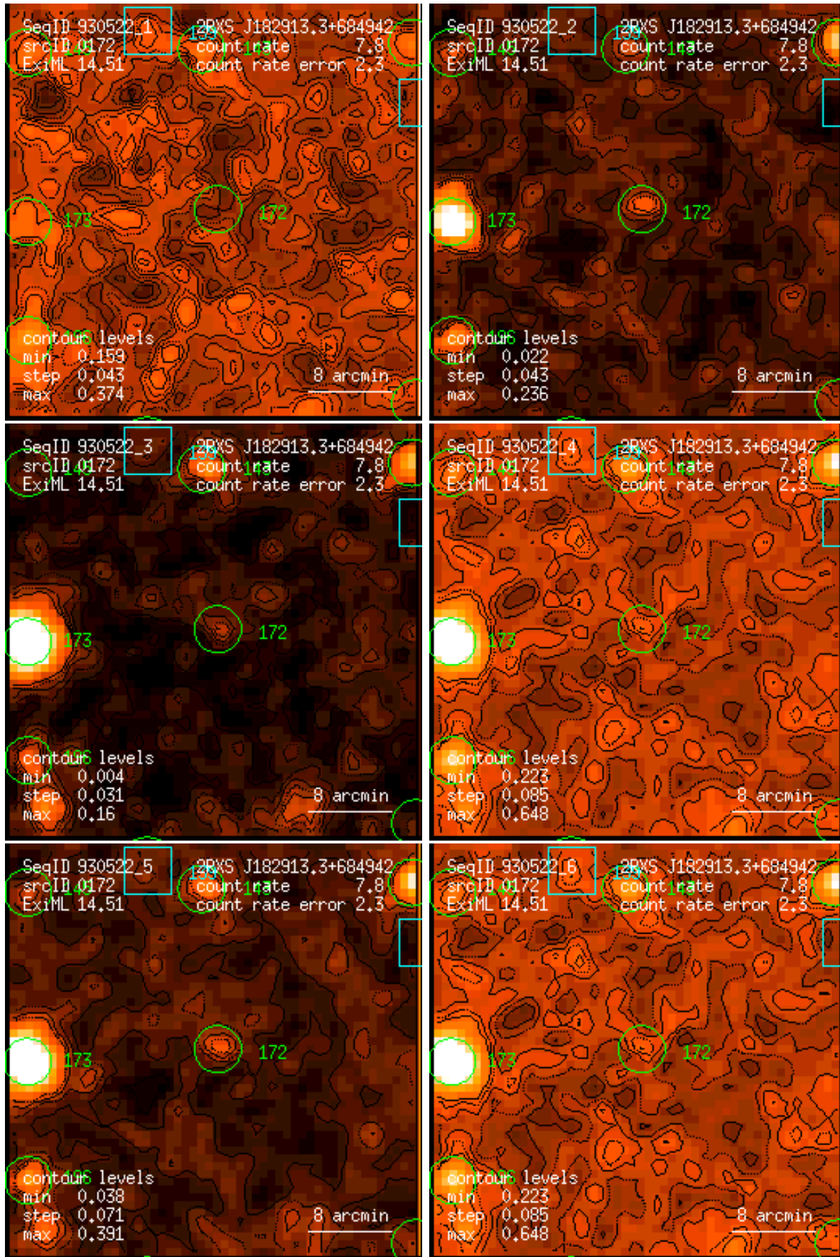
Figure 172: RASS 930522: detection 0172: band rate images, Gaussian filter: (1) PSPC channels 11 – 41, (2) 52 – 90, (3) 91 – 201, (4) 11 – 235, (5) 52 – 201, (6) 11 – 201. Broad band rates in counts/ks. Band rate contour levels in counts/ks/arcmin 2 .
