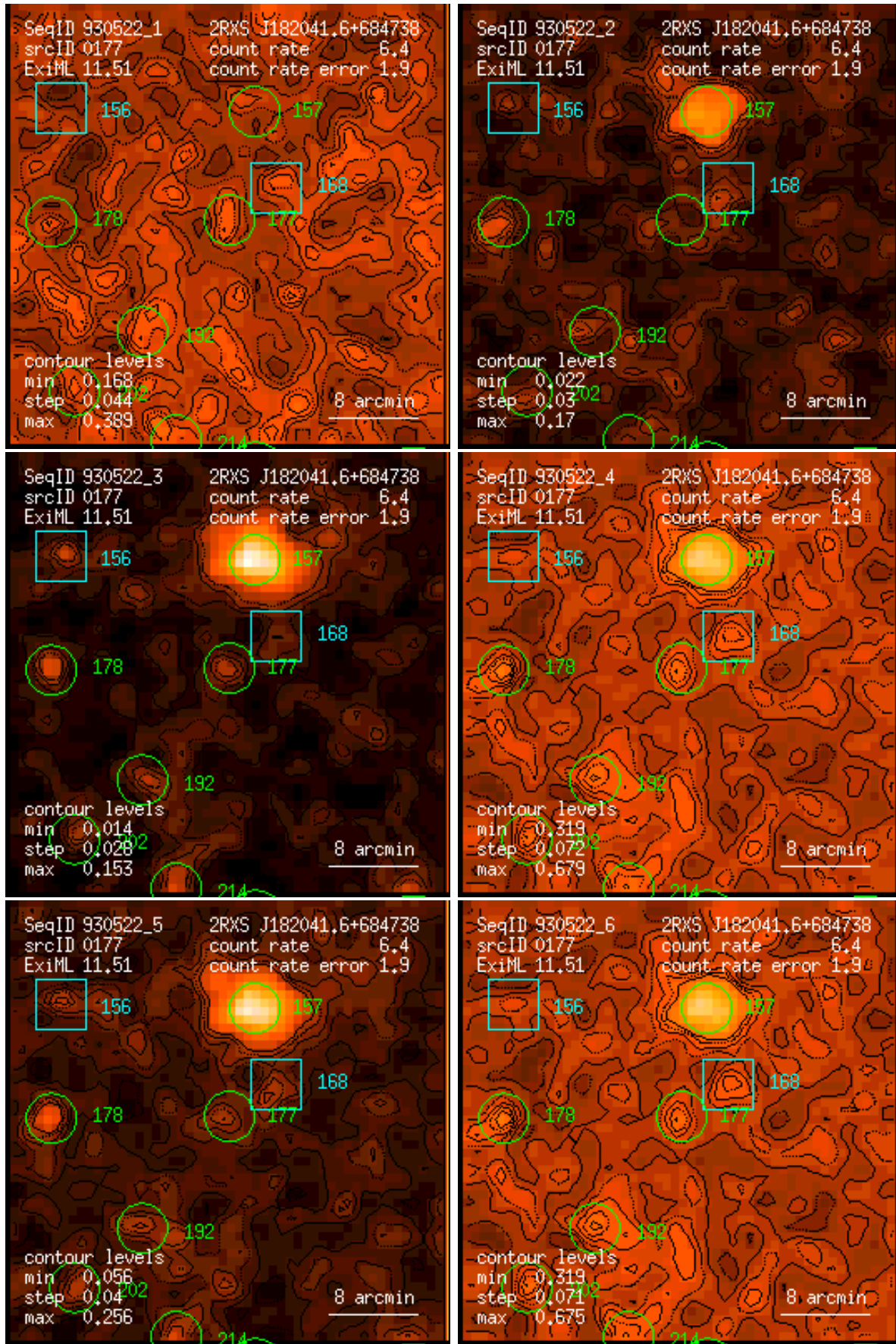
Figure 177: RASS 930522: detection 0177: band rate images, Gaussian filter: (1) PSPC channels 11 – 41, (2) 52 – 90, (3) 91 – 201, (4) 11 – 235, (5) 52 – 201, (6) 11 – 201. Broad band rates in counts/ks. Band rate contour levels in counts/ks/arcmin 2 .
