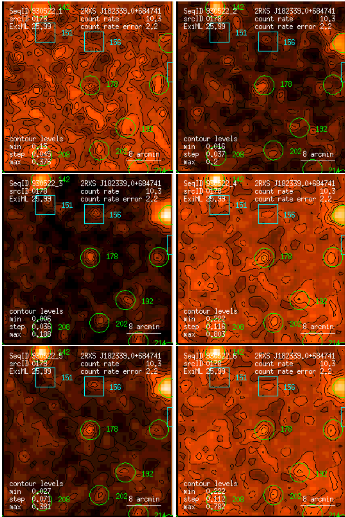
Figure 178: RASS 930522: detection 0178: band rate images, Gaussian filter: (1) PSPC channels 11 – 41, (2) 52 – 90, (3) 91 – 201, (4) 11 – 235, (5) 52 – 201, (6) 11 – 201. Broad band rates in counts/ks. Band rate contour levels in counts/ks/arcmin 2 .
