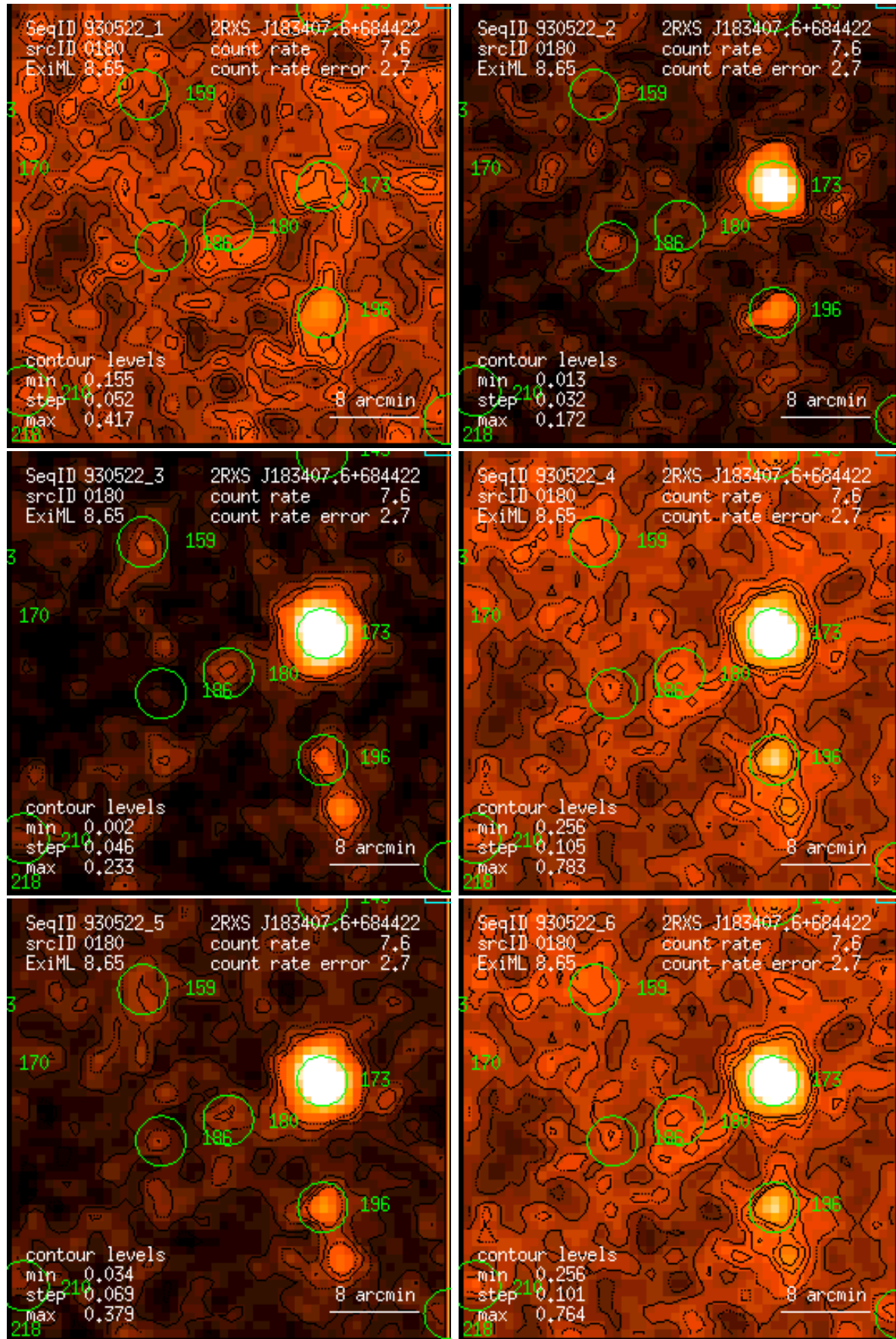
Figure 180: RASS 930522: detection 0180: band rate images, Gaussian filter: (1) PSPC channels 11 – 41, (2) 52 – 90, (3) 91 – 201, (4) 11 – 235, (5) 52 – 201, (6) 11 – 201. Broad band rates in counts/ks. Band rate contour levels in counts/ks/arcmin 2 .
