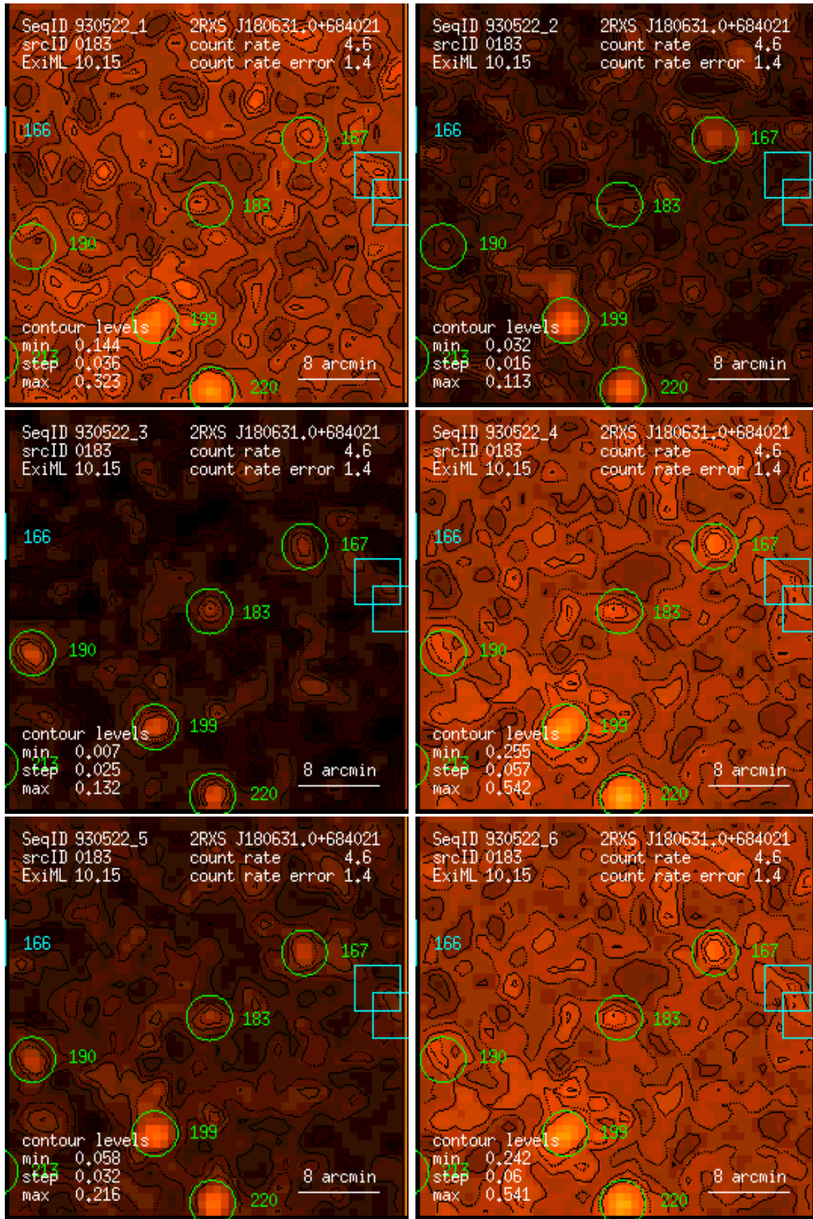
Figure 183: RASS 930522: detection 0183: band rate images, Gaussian filter: (1) PSPC channels 11 – 41, (2) 52 – 90, (3) 91 – 201, (4) 11 – 235, (5) 52 – 201, (6) 11 – 201. Broad band rates in counts/ks. Band rate contour levels in counts/ks/arcmin 2 .
