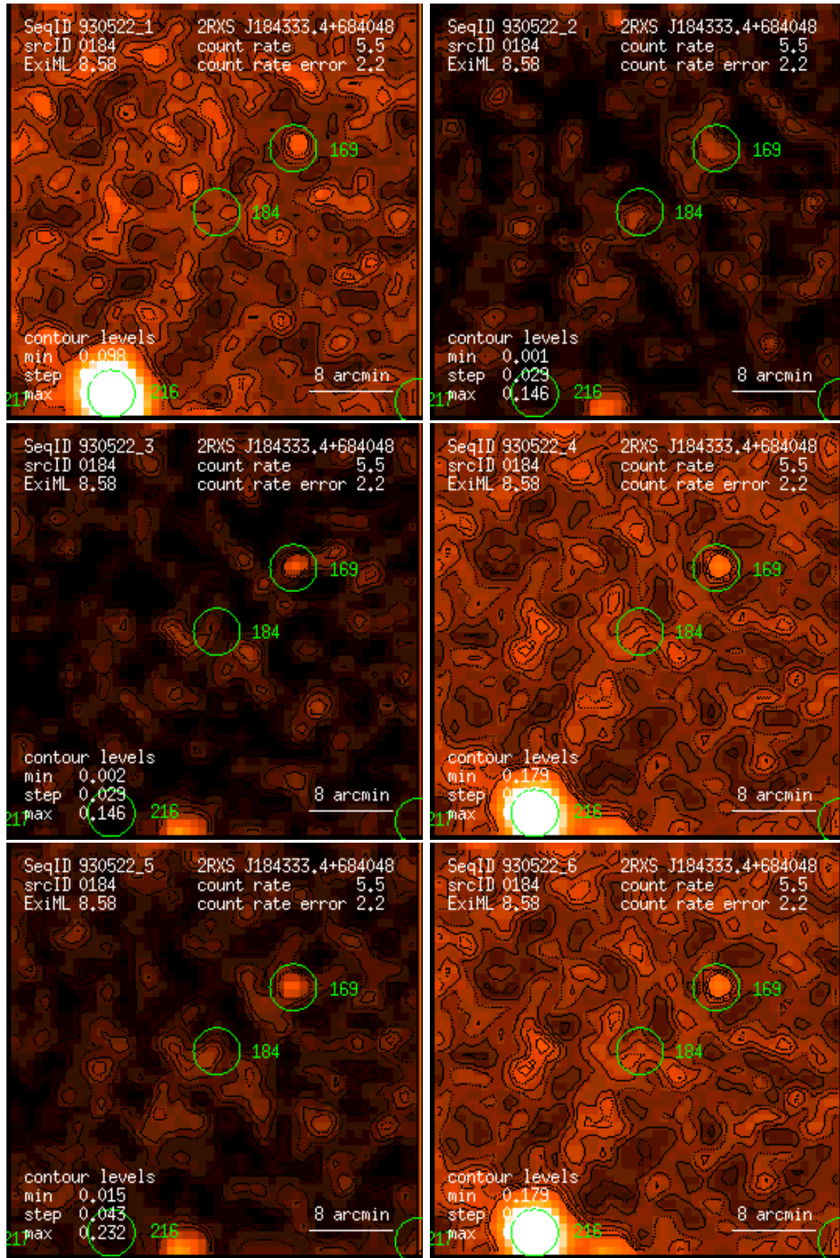
Figure 184: RASS 930522: detection 0184: band rate images, Gaussian filter: (1) PSPC channels 11 – 41, (2) 52 – 90, (3) 91 – 201, (4) 11 – 235, (5) 52 – 201, (6) 11 – 201. Broad band rates in counts/ks. Band rate contour levels in counts/ks/arcmin 2 .
