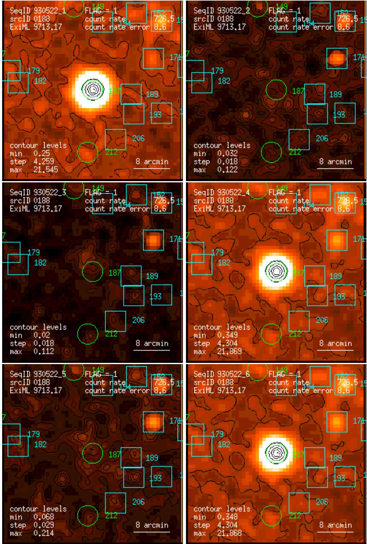
Figure 188: RASS 930522: detection 0188: band rate images, Gaussian filter: (1) PSPC channels 11 – 41, (2) 52 – 90, (3) 91 – 201, (4) 11 – 235, (5) 52 – 201, (6) 11 – 201. Broad band rates in counts/ks. Band rate contour levels in counts/ks/arcmin 2 .
