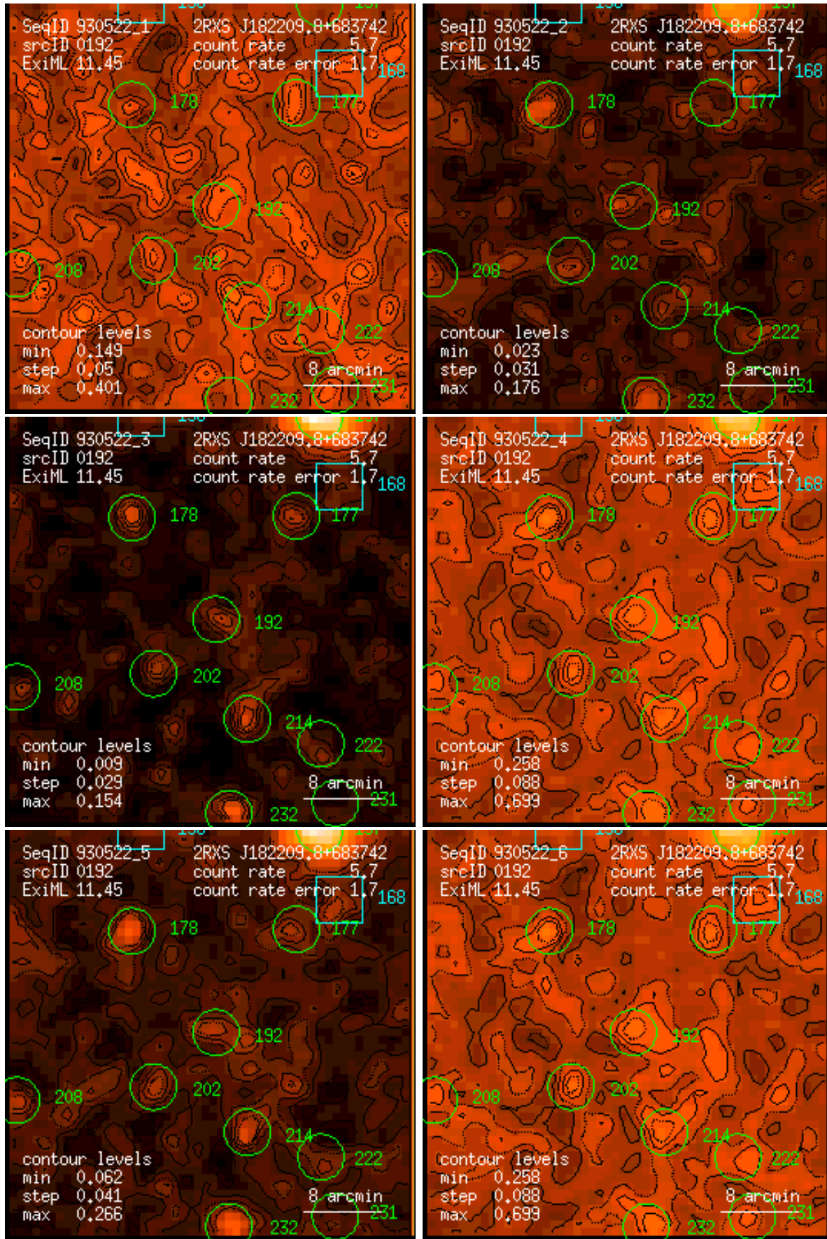
Figure 192: RASS 930522: detection 0192: band rate images, Gaussian filter: (1) PSPC channels 11 – 41, (2) 52 – 90, (3) 91 – 201, (4) 11 – 235, (5) 52 – 201, (6) 11 – 201. Broad band rates in counts/ks. Band rate contour levels in counts/ks/arcmin 2 .
