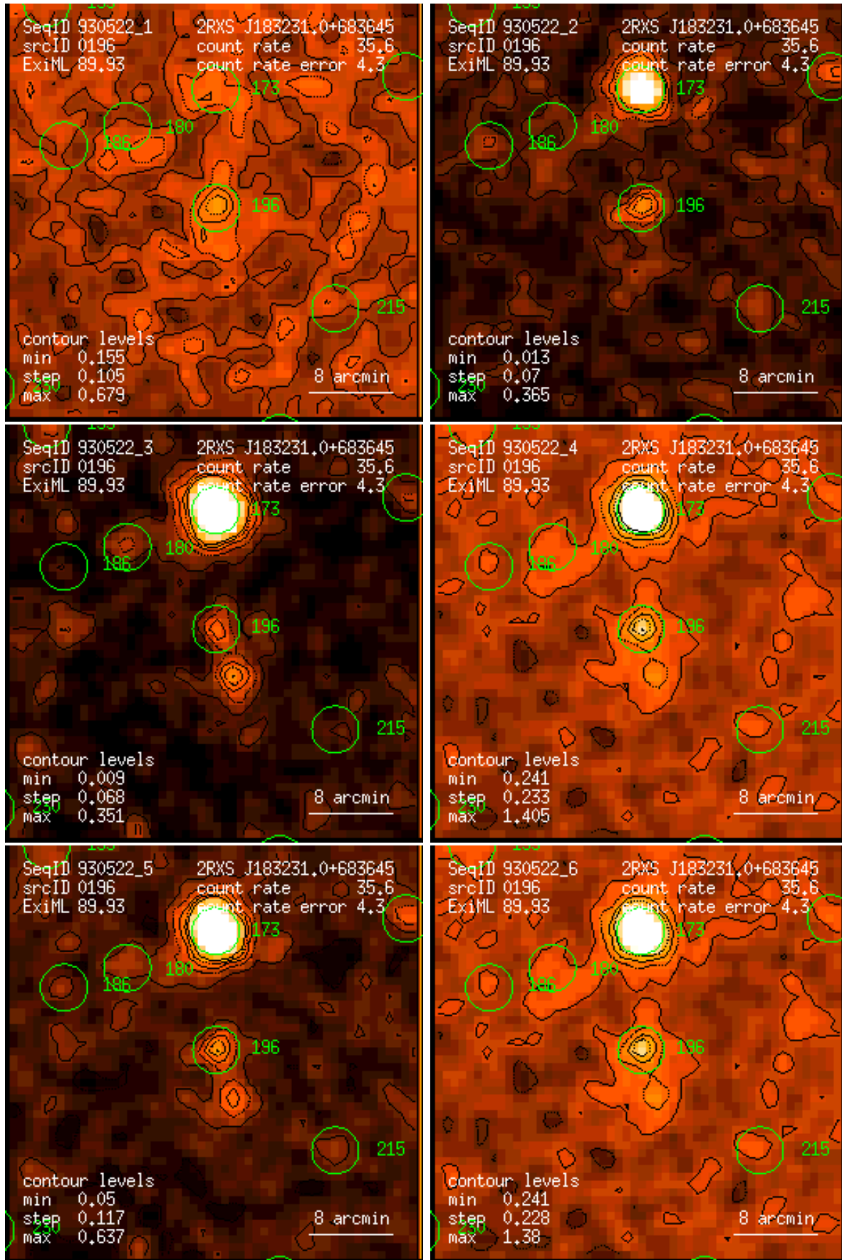
Figure 196: RASS 930522: detection 0196: band rate images, Gaussian filter: (1) PSPC channels 11 – 41, (2) 52 – 90, (3) 91 – 201, (4) 11 – 235, (5) 52 – 201, (6) 11 – 201. Broad band rates in counts/ks. Band rate contour levels in counts/ks/arcmin 2 .
