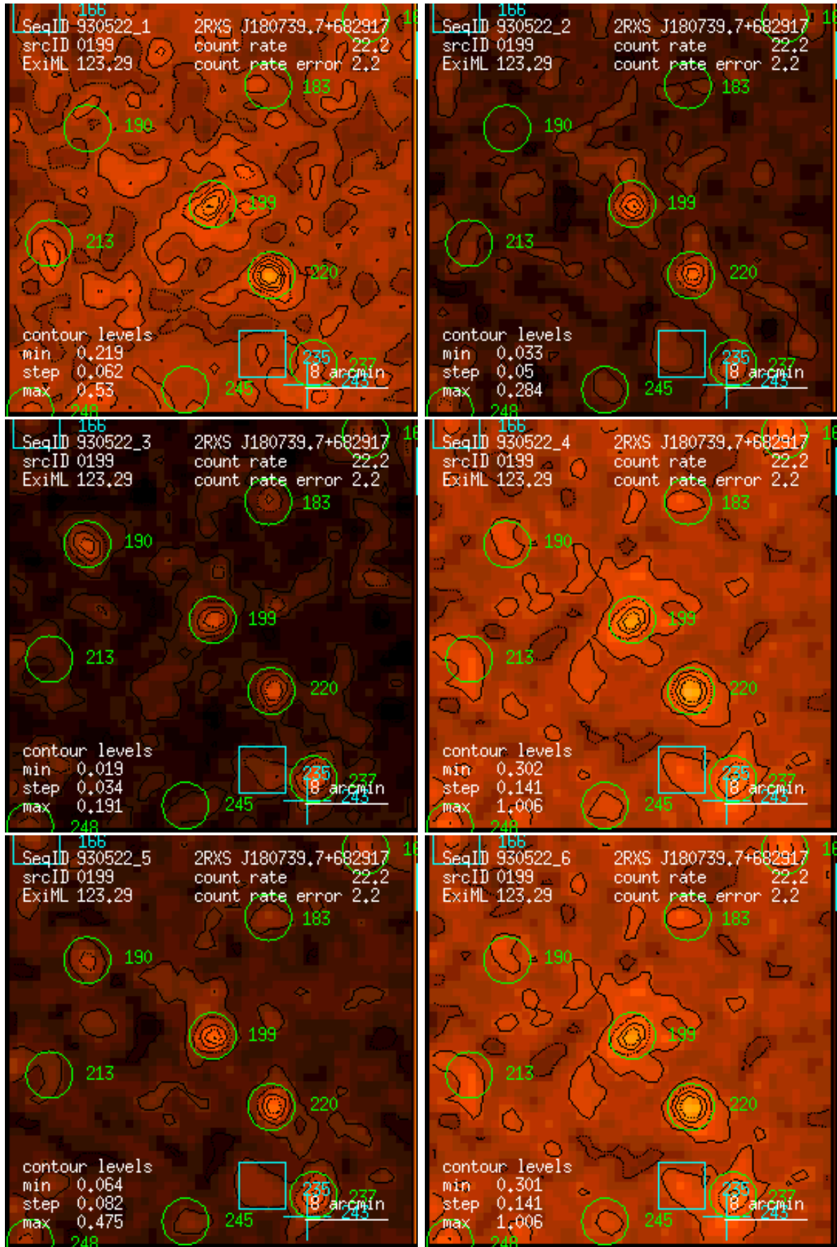
Figure 199: RASS 930522: detection 0199: band rate images, Gaussian filter: (1) PSPC channels 11 – 41, (2) 52 – 90, (3) 91 – 201, (4) 11 – 235, (5) 52 – 201, (6) 11 – 201. Broad band rates in counts/ks. Band rate contour levels in counts/ks/arcmin 2 .
