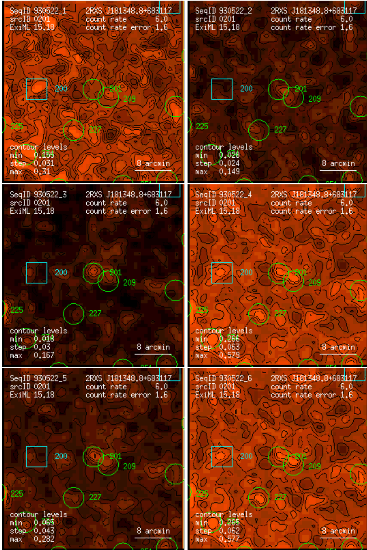
Figure 201: RASS 930522: detection 0201: band rate images, Gaussian filter: (1) PSPC channels 11 – 41, (2) 52 – 90, (3) 91 – 201, (4) 11 – 235, (5) 52 – 201, (6) 11 – 201. Broad band rates in counts/ks. Band rate contour levels in counts/ks/arcmin 2 .
