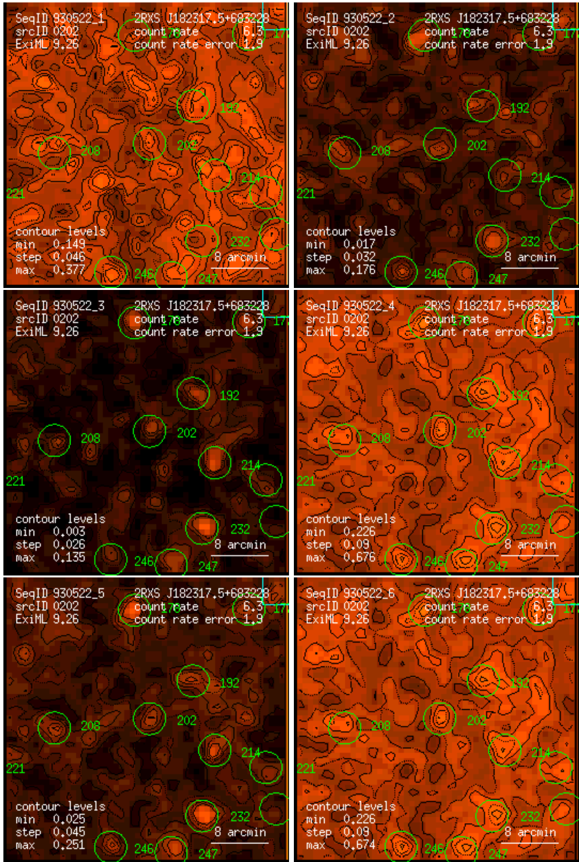
Figure 202: RASS 930522: detection 0202: band rate images, Gaussian filter: (1) PSPC channels 11 – 41, (2) 52 – 90, (3) 91 – 201, (4) 11 – 235, (5) 52 – 201, (6) 11 – 201. Broad band rates in counts/ks. Band rate contour levels in counts/ks/arcmin 2 .
