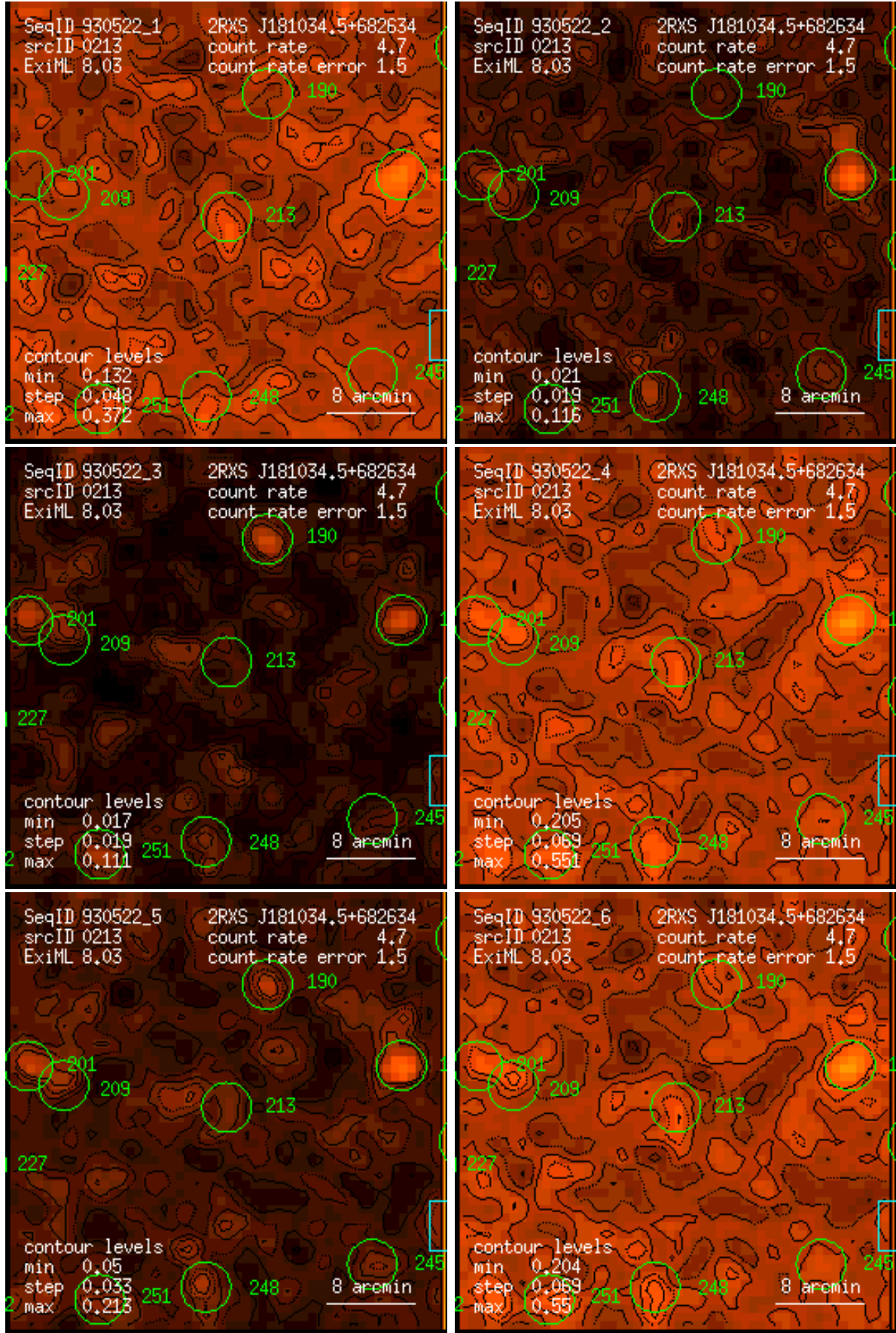
Figure 213: RASS 930522: detection 0213: band rate images, Gaussian filter: (1) PSPC channels 11 – 41, (2) 52 – 90, (3) 91 – 201, (4) 11 – 235, (5) 52 – 201, (6) 11 – 201. Broad band rates in counts/ks. Band rate contour levels in counts/ks/arcmin 2 .
