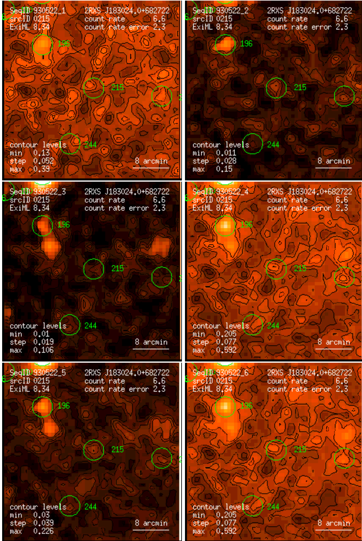
Figure 215: RASS 930522: detection 0215: band rate images, Gaussian filter: (1) PSPC channels 11 – 41, (2) 52 – 90, (3) 91 – 201, (4) 11 – 235, (5) 52 – 201, (6) 11 – 201. Broad band rates in counts/ks. Band rate contour levels in counts/ks/arcmin 2 .
