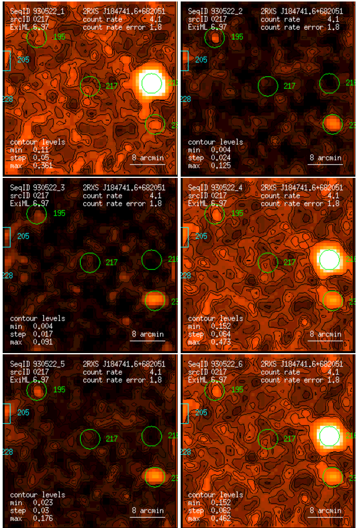
Figure 217: RASS 930522: detection 0217: band rate images, Gaussian filter: (1) PSPC channels 11 – 41, (2) 52 – 90, (3) 91 – 201, (4) 11 – 235, (5) 52 – 201, (6) 11 – 201. Broad band rates in counts/ks. Band rate contour levels in counts/ks/arcmin 2 .
