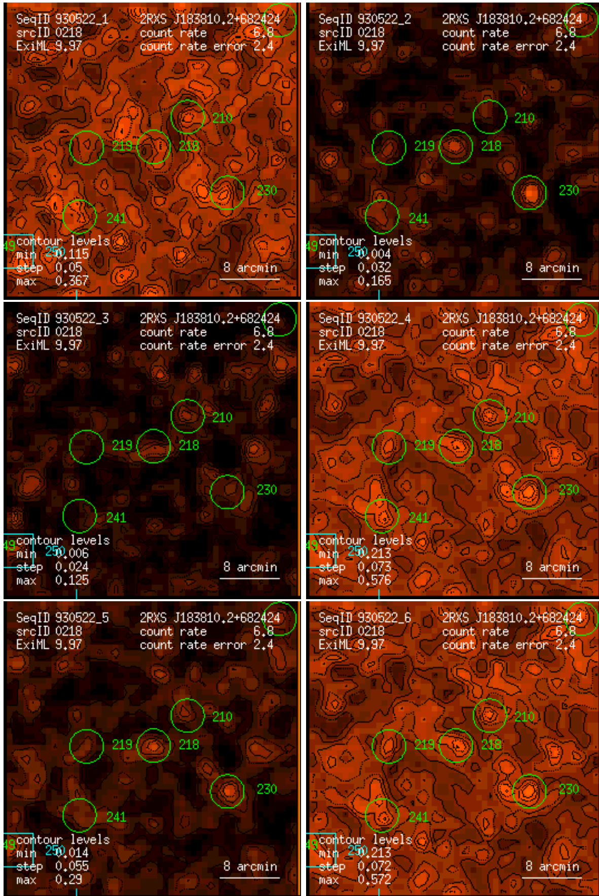
Figure 218: RASS 930522: detection 0218: band rate images, Gaussian filter: (1) PSPC channels 11 – 41, (2) 52 – 90, (3) 91 – 201, (4) 11 – 235, (5) 52 – 201, (6) 11 – 201. Broad band rates in counts/ks. Band rate contour levels in counts/ks/arcmin 2 .
