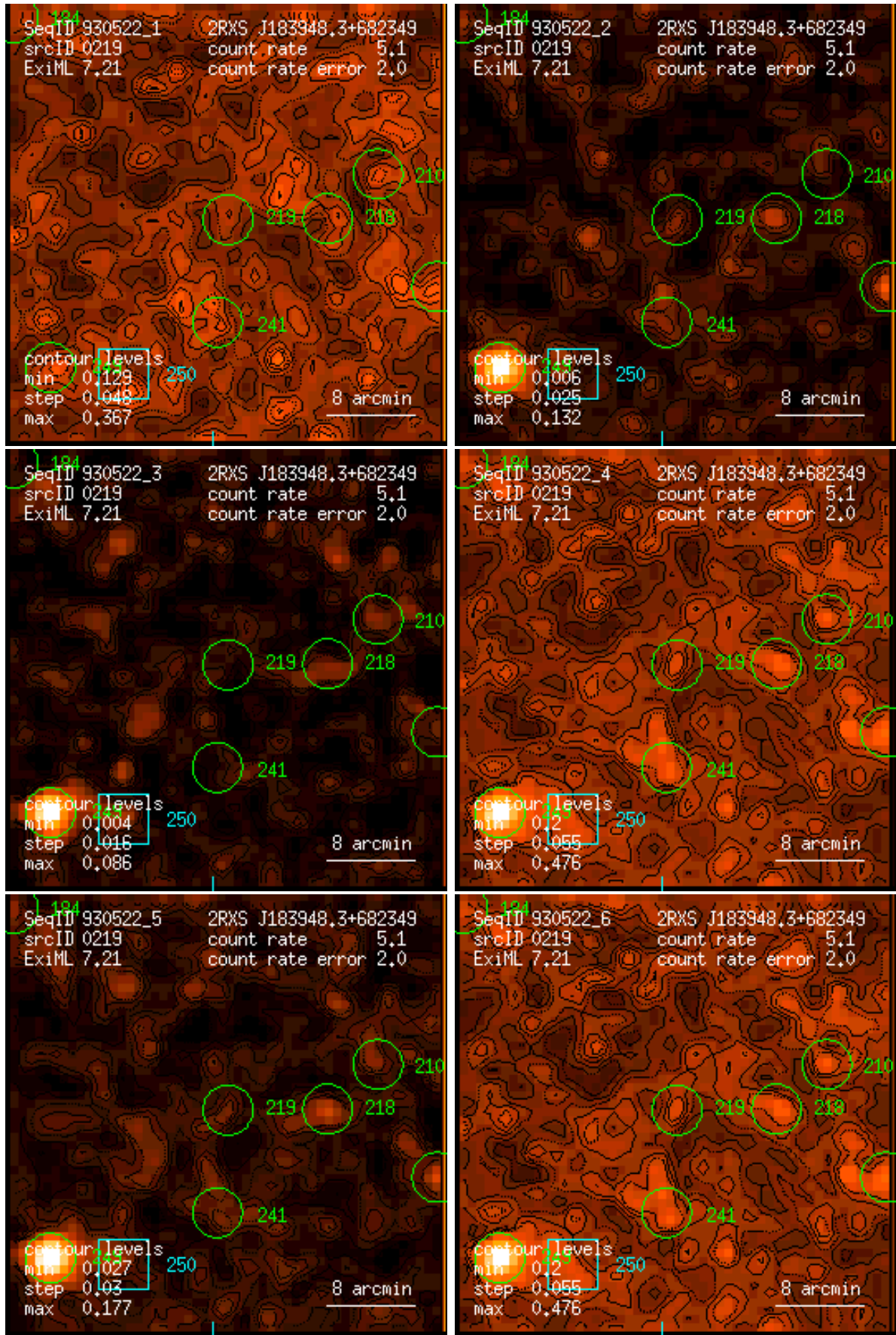
Figure 219: RASS 930522: detection 0219: band rate images, Gaussian filter: (1) PSPC channels 11 – 41, (2) 52 – 90, (3) 91 – 201, (4) 11 – 235, (5) 52 – 201, (6) 11 – 201. Broad band rates in counts/ks. Band rate contour levels in counts/ks/arcmin 2 .
