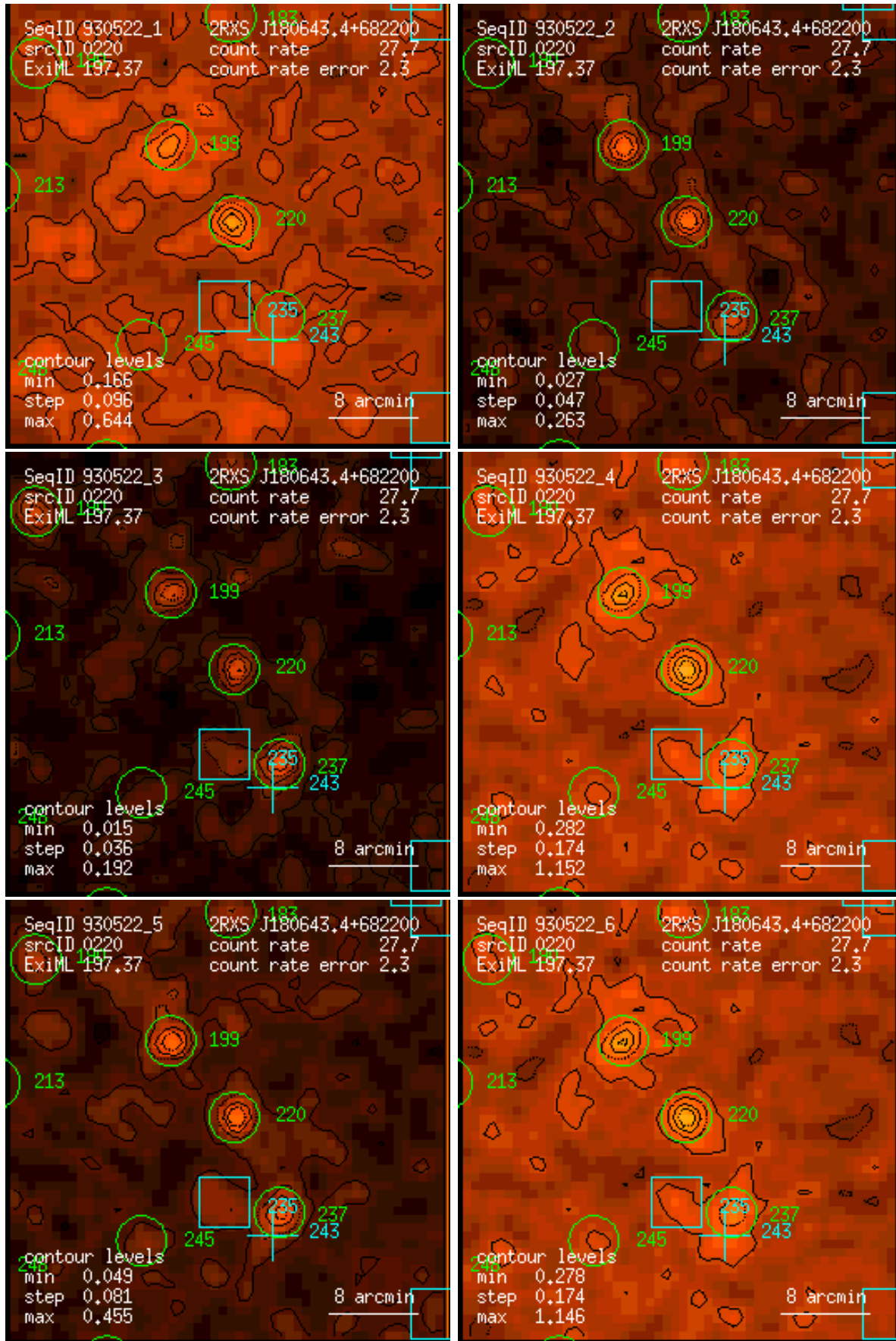
Figure 220: RASS 930522: detection 0220: band rate images, Gaussian filter: (1) PSPC channels 11 – 41, (2) 52 – 90, (3) 91 – 201, (4) 11 – 235, (5) 52 – 201, (6) 11 – 201. Broad band rates in counts/ks. Band rate contour levels in counts/ks/arcmin 2 .
