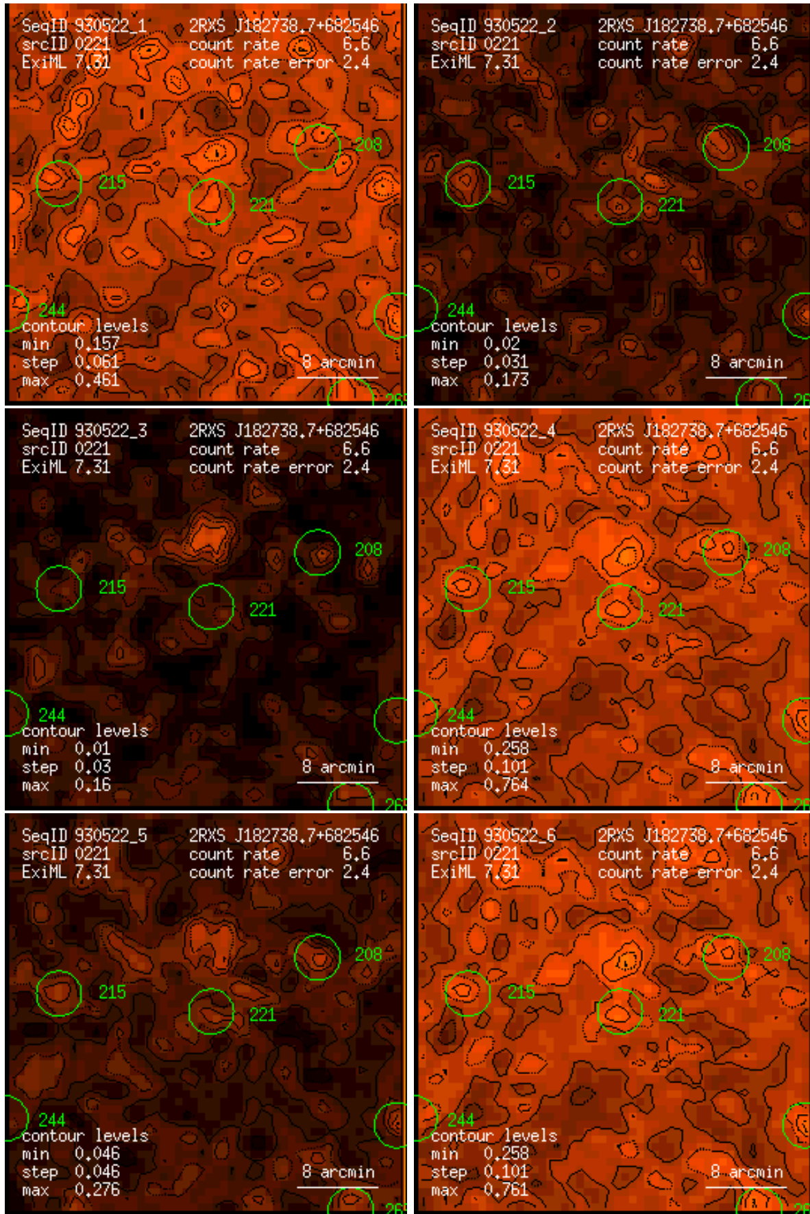
Figure 221: RASS 930522: detection 0221: band rate images, Gaussian filter: (1) PSPC channels 11 – 41, (2) 52 – 90, (3) 91 – 201, (4) 11 – 235, (5) 52 – 201, (6) 11 – 201. Broad band rates in counts/ks. Band rate contour levels in counts/ks/arcmin 2 .
