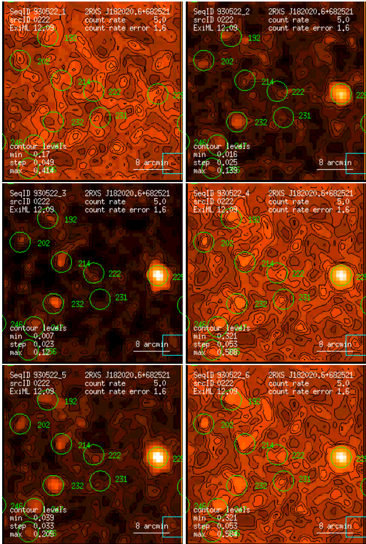
Figure 222: RASS 930522: detection 0222: band rate images, Gaussian filter: (1) PSPC channels 11 – 41, (2) 52 – 90, (3) 91 – 201, (4) 11 – 235, (5) 52 – 201, (6) 11 – 201. Broad band rates in counts/ks. Band rate contour levels in counts/ks/arcmin 2 .
