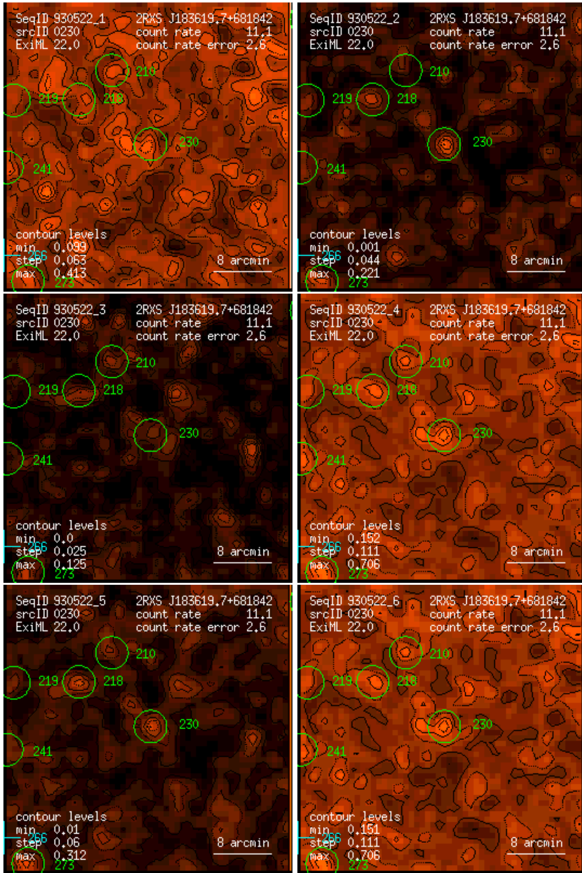
Figure 230: RASS 930522: detection 0230: band rate images, Gaussian filter: (1) PSPC channels 11 – 41, (2) 52 – 90, (3) 91 – 201, (4) 11 – 235, (5) 52 – 201, (6) 11 – 201. Broad band rates in counts/ks. Band rate contour levels in counts/ks/arcmin 2 .
