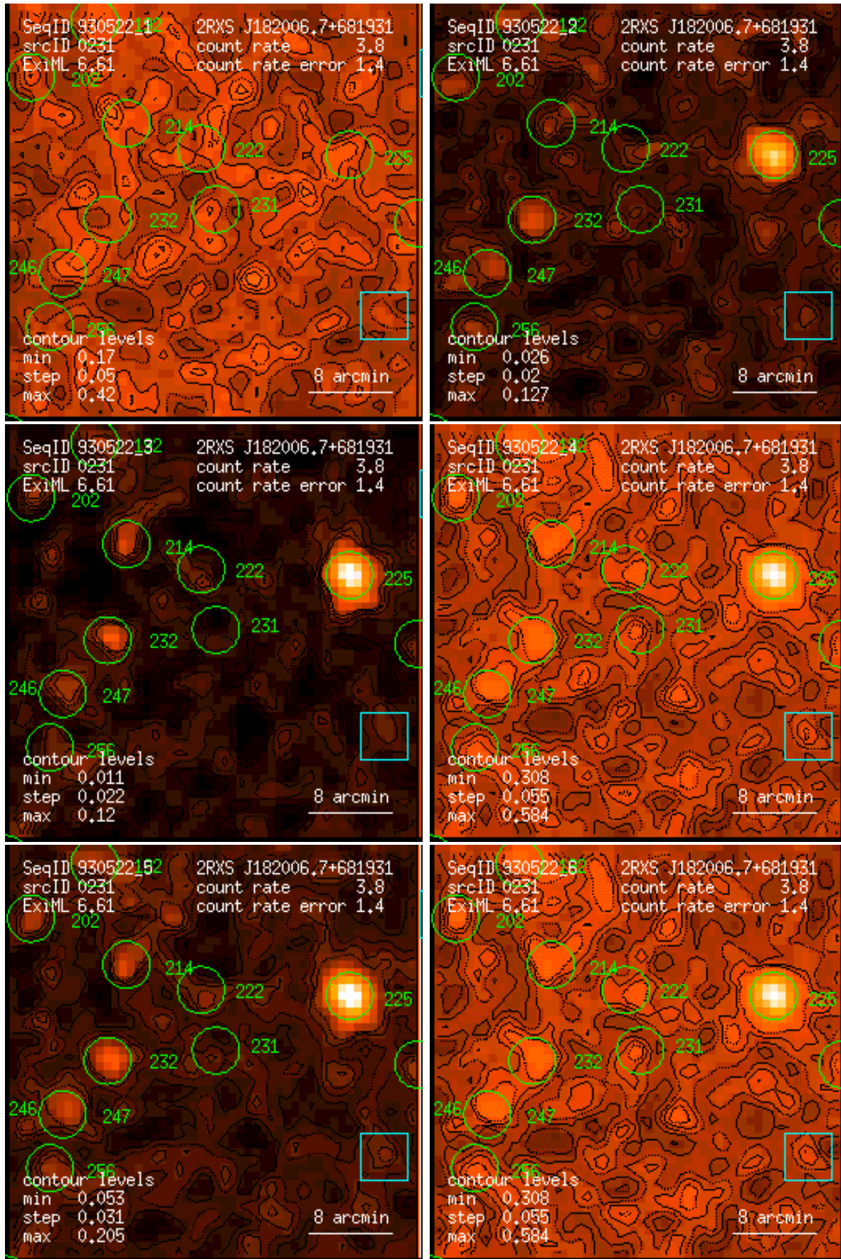
Figure 231: RASS 930522: detection 0231: band rate images, Gaussian filter: (1) PSPC channels 11 – 41, (2) 52 – 90, (3) 91 – 201, (4) 11 – 235, (5) 52 – 201, (6) 11 – 201. Broad band rates in counts/ks. Band rate contour levels in counts/ks/arcmin 2 .
