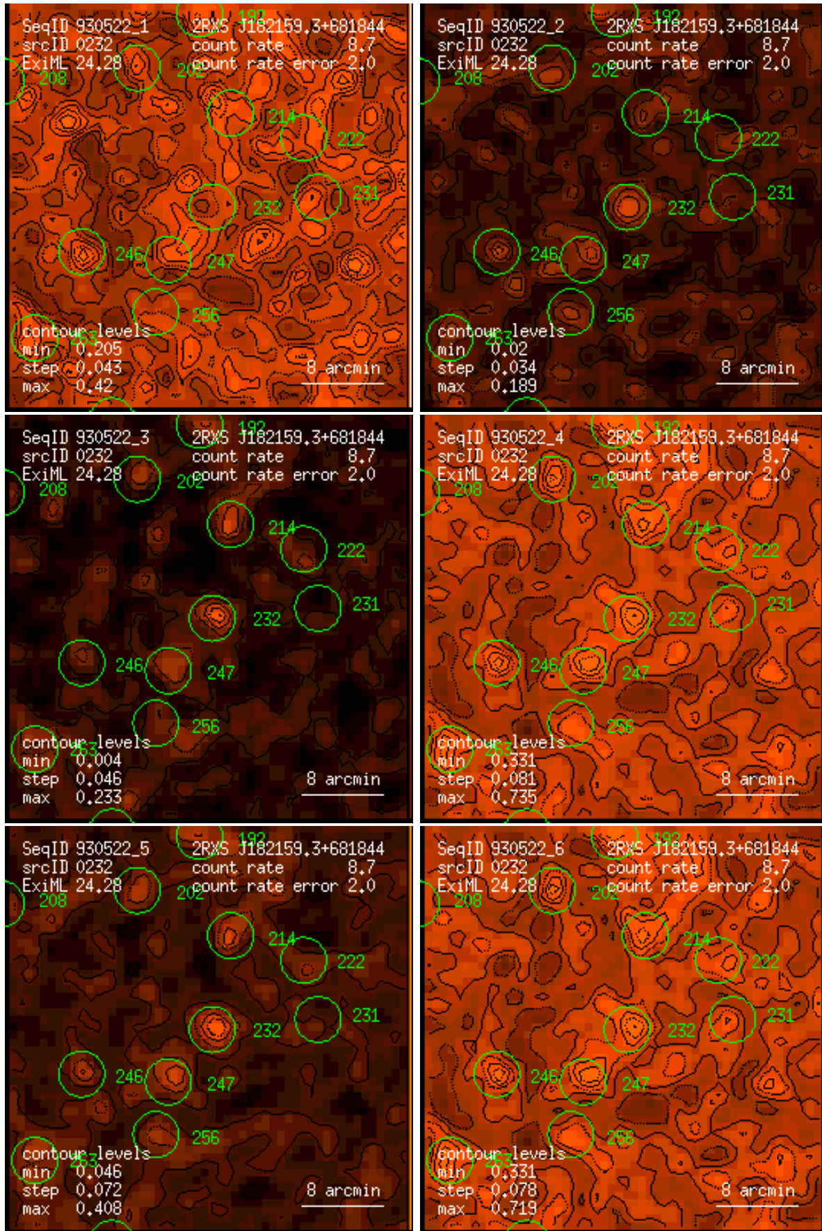
Figure 232: RASS 930522: detection 0232: band rate images, Gaussian filter: (1) PSPC channels 11 – 41, (2) 52 – 90, (3) 91 – 201, (4) 11 – 235, (5) 52 – 201, (6) 11 – 201. Broad band rates in counts/ks. Band rate contour levels in counts/ks/arcmin 2 .
