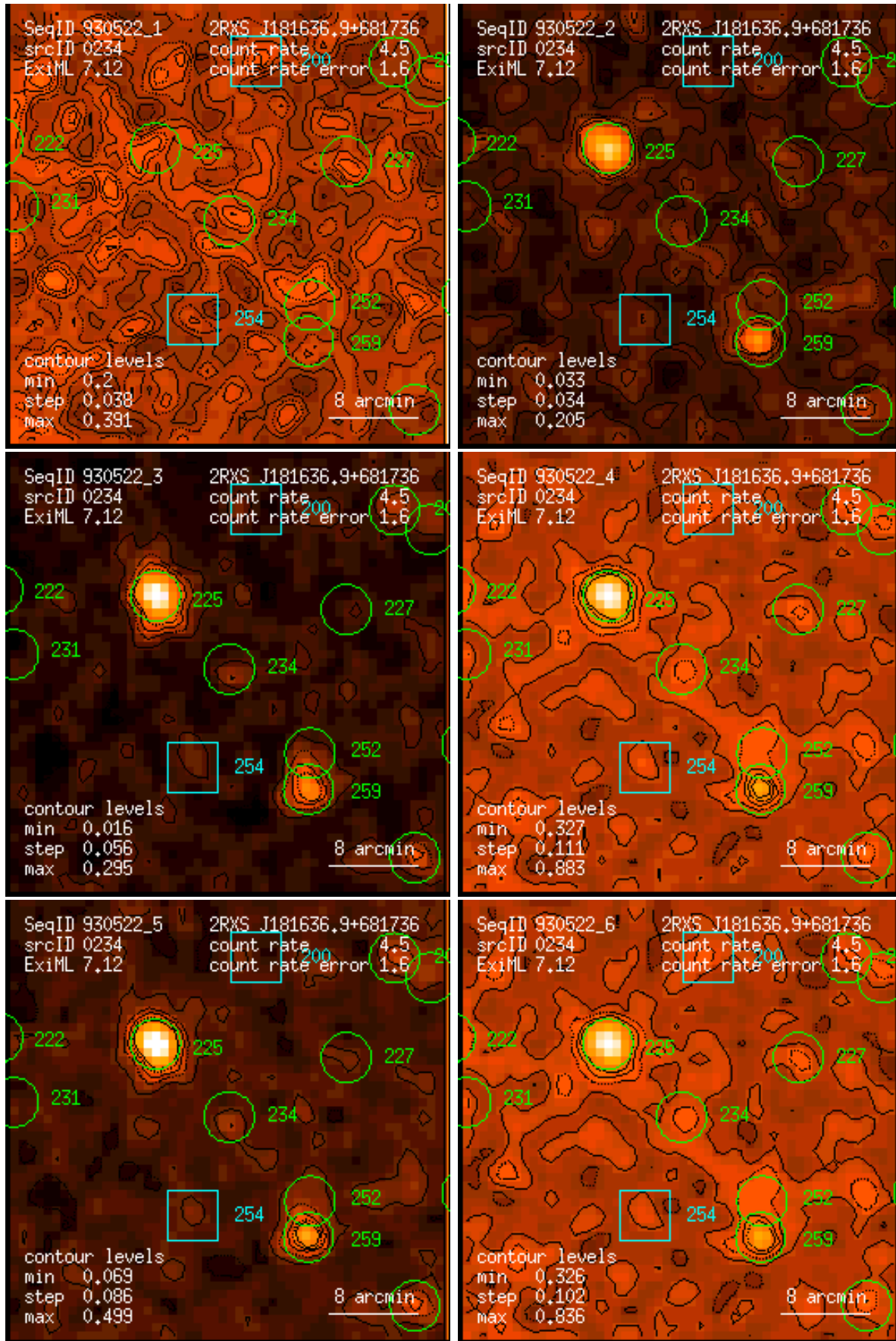
Figure 234: RASS 930522: detection 0234: band rate images, Gaussian filter: (1) PSPC channels 11 – 41, (2) 52 – 90, (3) 91 – 201, (4) 11 – 235, (5) 52 – 201, (6) 11 – 201. Broad band rates in counts/ks. Band rate contour levels in counts/ks/arcmin 2 .
