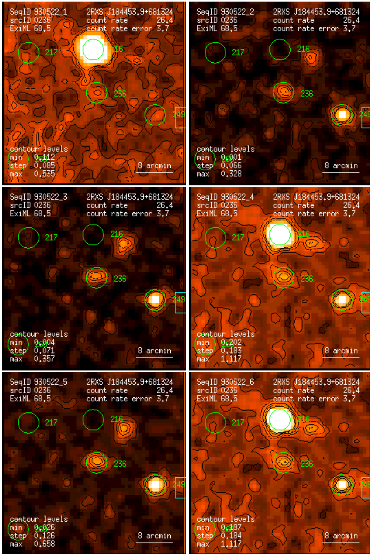
Figure 236: RASS 930522: detection 0236: band rate images, Gaussian filter: (1) PSPC channels 11 – 41, (2) 52 – 90, (3) 91 – 201, (4) 11 – 235, (5) 52 – 201, (6) 11 – 201. Broad band rates in counts/ks. Band rate contour levels in counts/ks/arcmin 2 .
