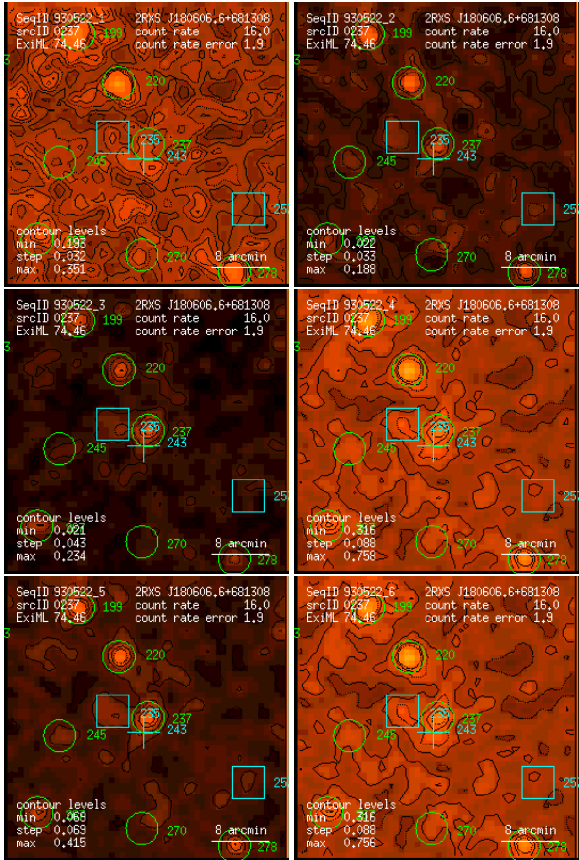
Figure 237: RASS 930522: detection 0237: band rate images, Gaussian filter: (1) PSPC channels 11 – 41, (2) 52 – 90, (3) 91 – 201, (4) 11 – 235, (5) 52 – 201, (6) 11 – 201. Broad band rates in counts/ks. Band rate contour levels in counts/ks/arcmin 2 .
