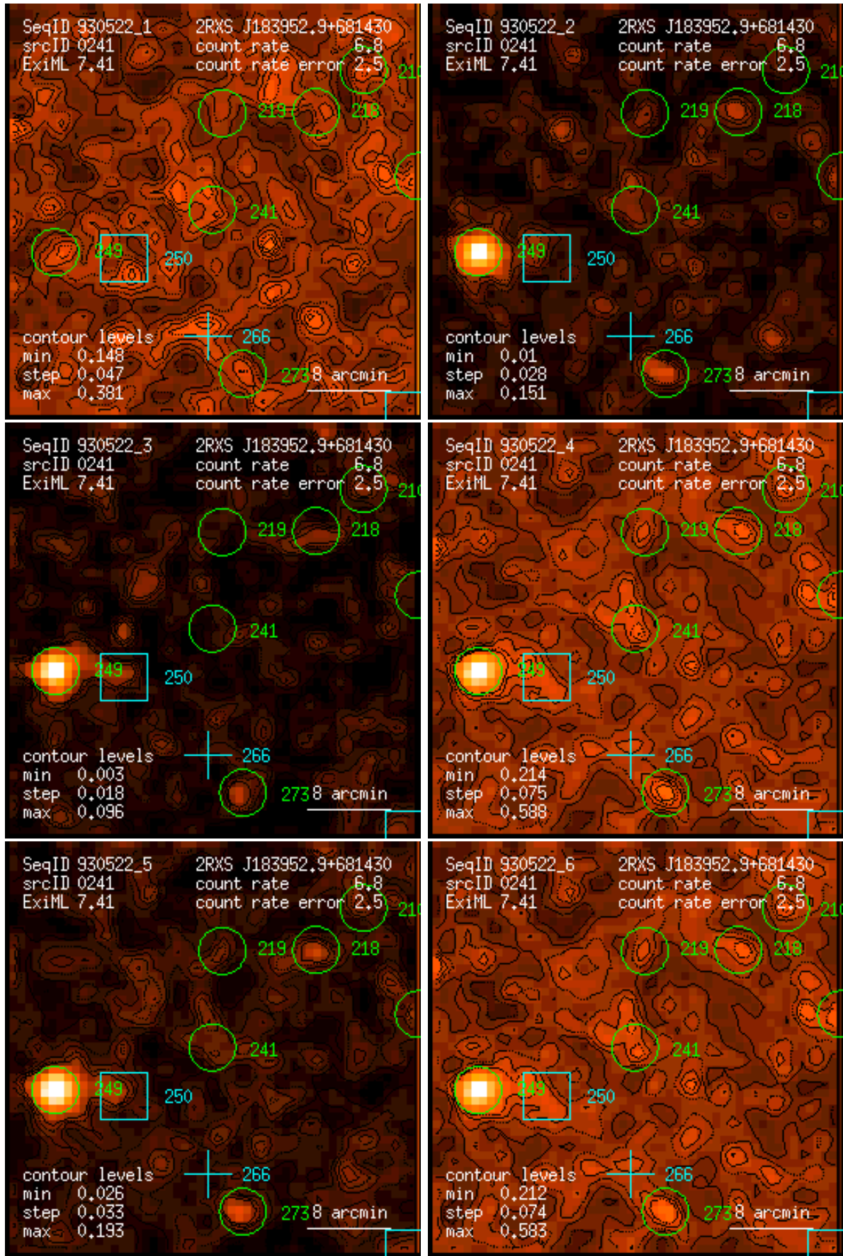
Figure 241: RASS 930522: detection 0241: band rate images, Gaussian filter: (1) PSPC channels 11 – 41, (2) 52 – 90, (3) 91 – 201, (4) 11 – 235, (5) 52 – 201, (6) 11 – 201. Broad band rates in counts/ks. Band rate contour levels in counts/ks/arcmin 2 .
