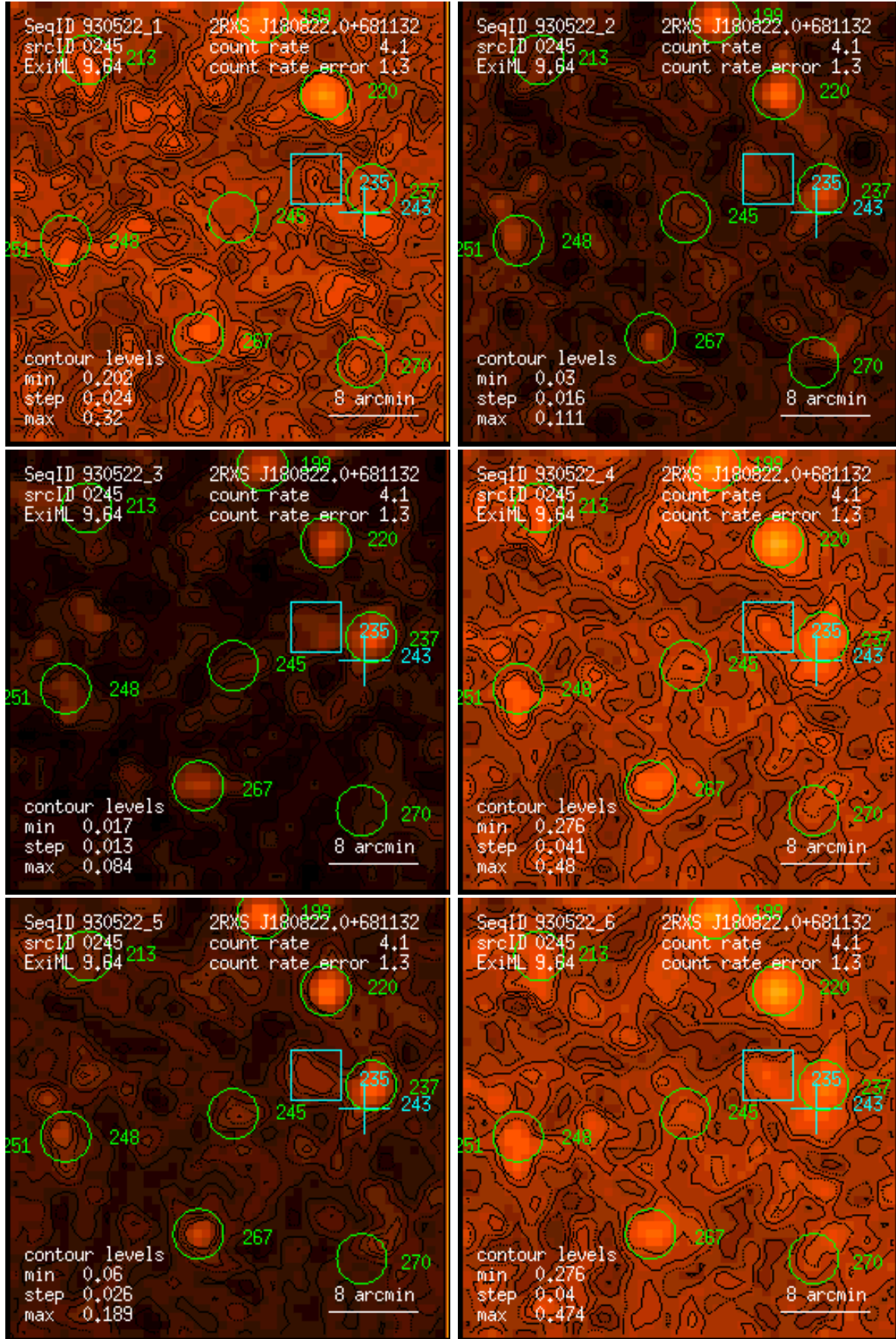
Figure 245: RASS 930522: detection 0245: band rate images, Gaussian filter: (1) PSPC channels 11 – 41, (2) 52 – 90, (3) 91 – 201, (4) 11 – 235, (5) 52 – 201, (6) 11 – 201. Broad band rates in counts/ks. Band rate contour levels in counts/ks/arcmin 2 .
