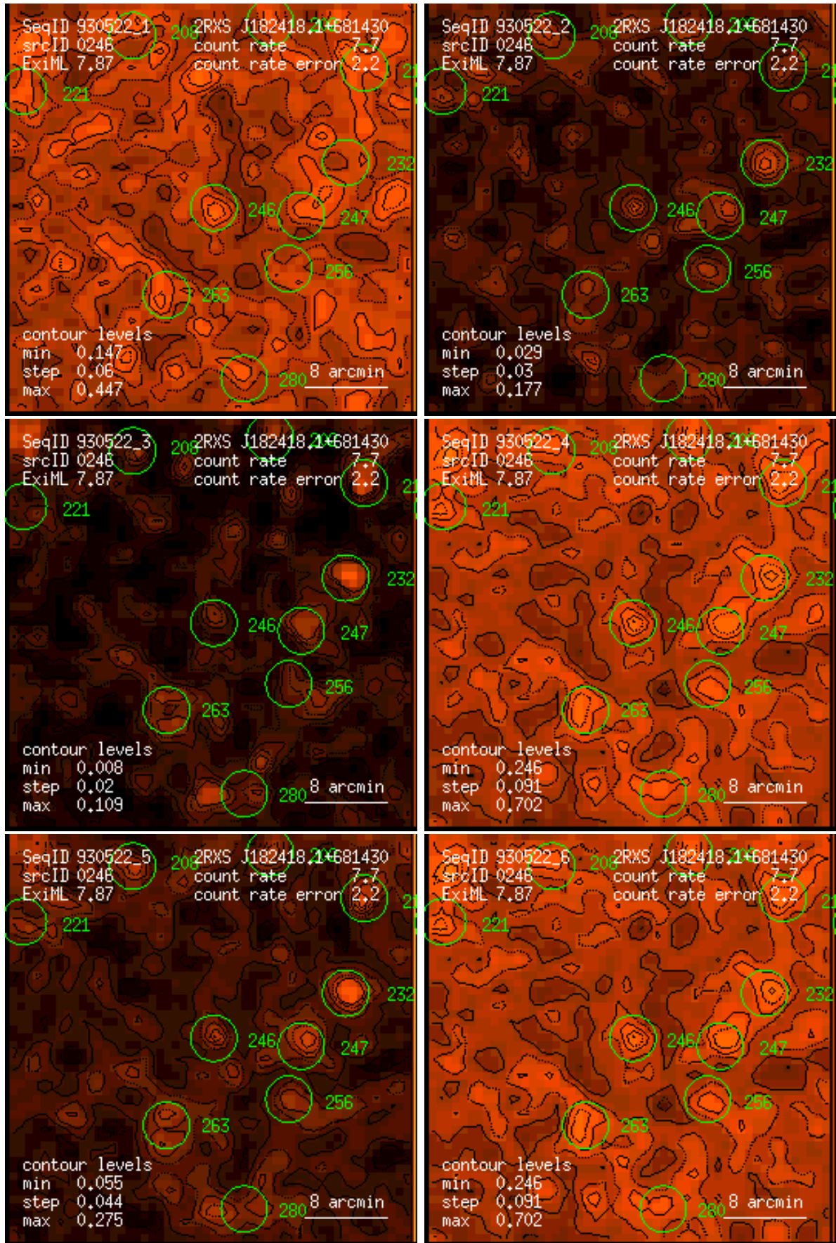
Figure 246: RASS 930522: detection 0246: band rate images, Gaussian filter: (1) PSPC channels 11 – 41, (2) 52 – 90, (3) 91 – 201, (4) 11 – 235, (5) 52 – 201, (6) 11 – 201. Broad band rates in counts/ks. Band rate contour levels in counts/ks/arcmin 2 .
